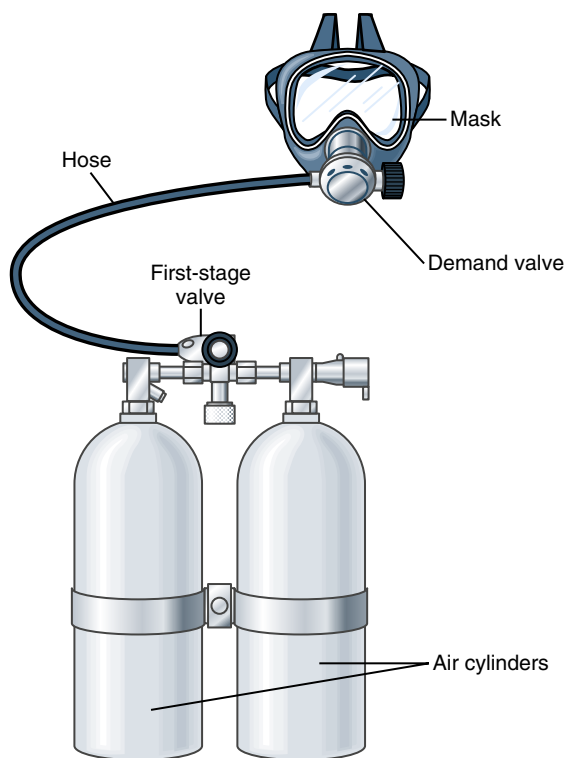
Figure 45-4. Open-circuit demand type of SCUBA (self-contained underwater breathing apparatus).
