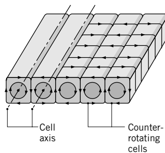
FIGURE 9.11 Longitudinal roll cells characteristic of advection in a horizontal fluid layer heated from below ( 1708 < Ra_L \lesssim 5 \times 10^4 ).
