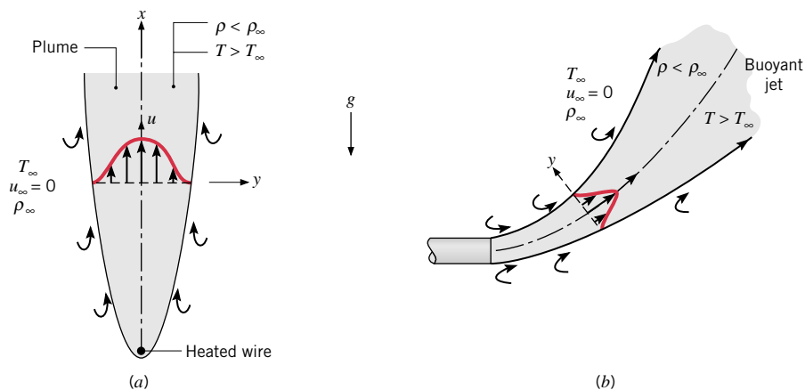
FIGURE 9.2 Buoyancy-driven free boundary layer flows in an extensive, quiescent medium. (a) Plume formation above a heated wire. (b) Buoyant jet associated with a heated discharge.
