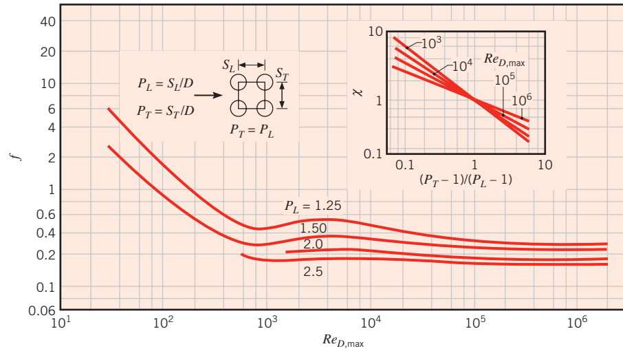
FIGURE 7.14 Friction factor f and correction factor \chi for Equation 7.65. In-line tube bundle arrangement [16]. (Used with permission.)
