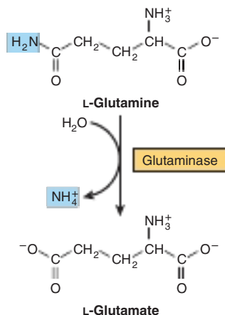
FIGURE 28–15 The reaction catalyzed by glutaminase, EC 3.5.1.2 . The reaction proceeds essentially irreversibly in the direction of glutamate and NH 4 + formation. Note that the amide nitrogen, not the \alpha -amino nitrogen, is removed.
