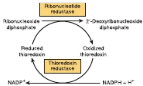
FIGURE 33-7 Reduction of ribonucleoside diphosphates to 2'-deoxyribonucleoside diphosphates.
