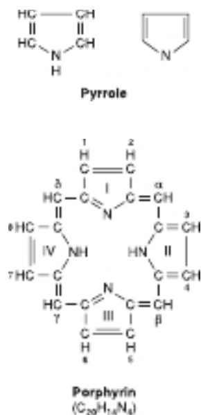
FIGURE 31-1 The porphyrin molecule. Rings are labeled I, II, III, and IV. Substituent positions are labeled 1 through 8. The four methylene bridges (=HC—) are labeled \alpha , \beta , \gamma , and \delta .
