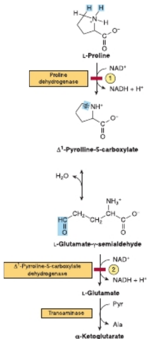
FIGURE 29–2 Catabolism of proline. Red bars and circled numerals indicate the locus of the inherited metabolic defects in 1 type-I hyperprolinemia and 2 type-II hyperprolinemia. In this and subsequent figures, blue highlights emphasize the portions of the molecules that are undergoing chemical change.
