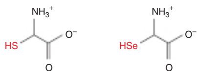
FIGURE 3–1 Cysteine (left) and selenocysteine (right). pK_a for the selenyl proton of selenocysteine is 5.2. Since this is 3 pH units lower than that of cysteine, selenocysteine represents a better nucleophile at or below pH 7.4.
