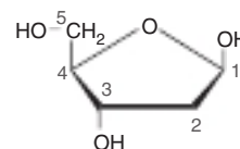
FIGURE 15-9 2-Deoxy-D-ribofuranose ( \beta -form).
