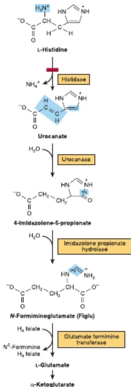
FIGURE 29-4 Catabolism of L-histidine to \alpha -ketoglutarate. ( \text{H}_4 folate, tetrahydrofolate.) The red bar indicates the site of an inherited metabolic defect.
