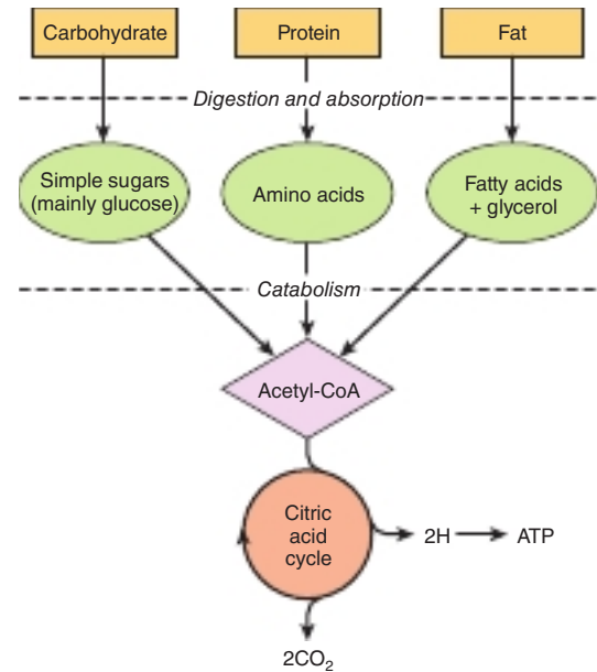
FIGURE 14-2 Outline of the pathways for the catabolism of carbohydrate, protein, and fat. All these pathways lead to the production of acetyl-CoA, which is oxidized in the citric acid cycle, ultimately yielding ATP by the process of oxidative phosphorylation.
