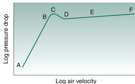
Fig. 30.3 Effect of air velocity on pressure drop through a fluidized bed.
