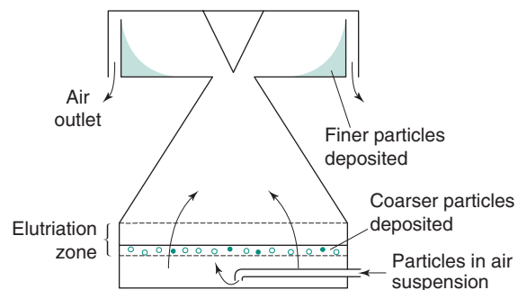
Fig. 10.20 Upward airflow elutriator.
