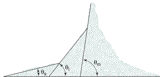
Fig. 12.1 Cohesive powder poured in a heap and showing different angles of repose: \theta_m , maximum angle formed by cohesive particles; \theta_s , shallowest angle formed by collapse of the cohesive particle heap, resulting in flooding. In some cases, a third angle, \theta_i , is identifiable as an intermediate slope produced by cohesive particles stacking on flooded powder.
