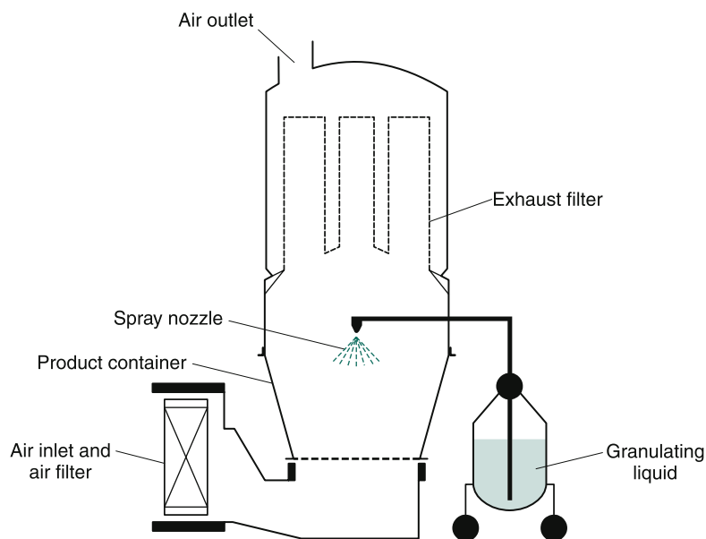
Fig. 29.7 Fluidized-bed granulator.
