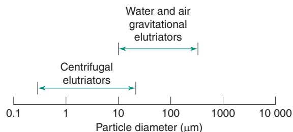
Fig. 10.18 Separation range for elutriation methods.
