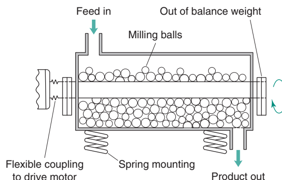
Fig. 10.9 Vibration mill.
