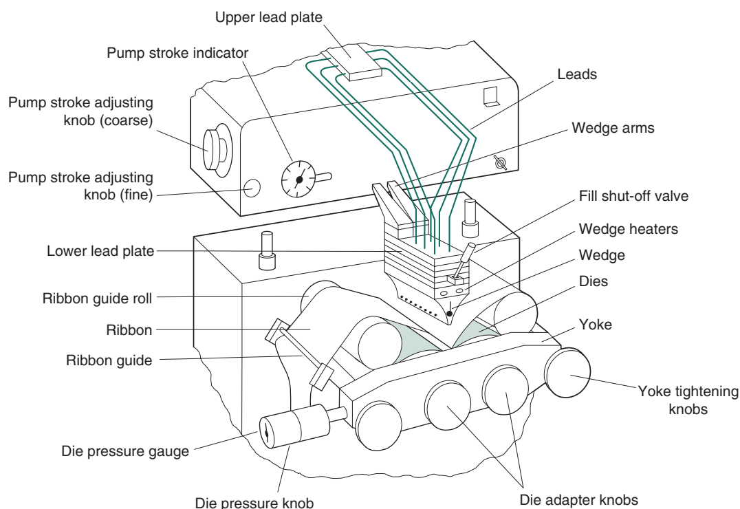
Fig. 36.4 Detail of capsule forming and filling elements of a soft capsule encapsulation machine.
