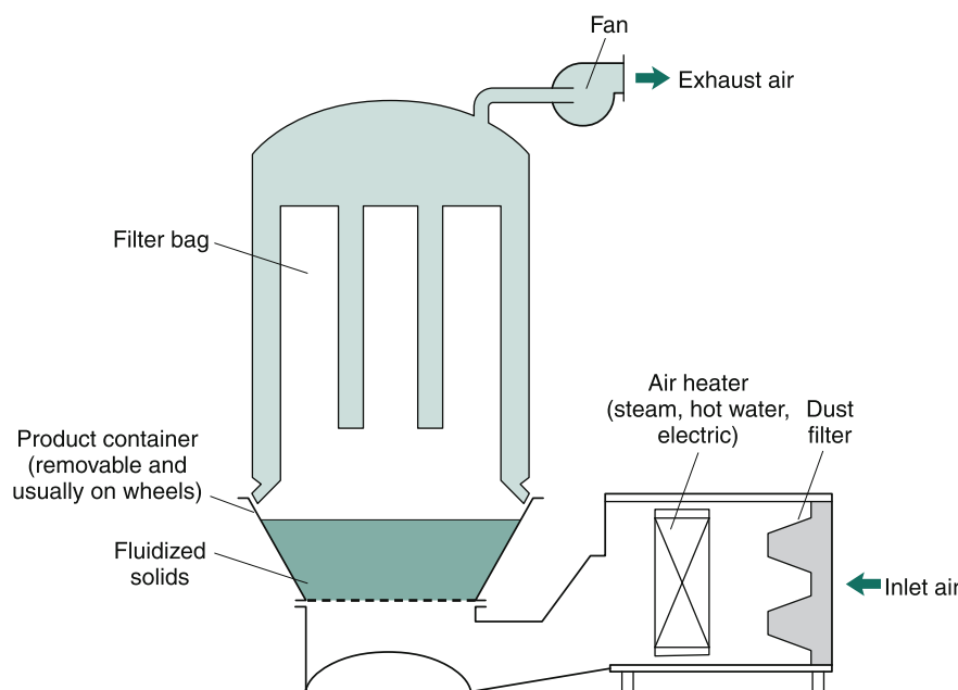
Fig. 30.4 Fluidized-bed dryer.
