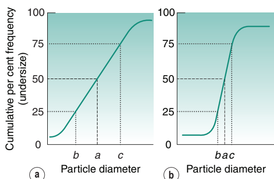
Fig. 9.5 Cumulative-frequency distribution curves. Point a corresponds to the median diameter; b is the lower quartile point and c is the upper quartile point. Plot (a) is for particles having a wide size distribution and (b) is for a narrow size distribution.
