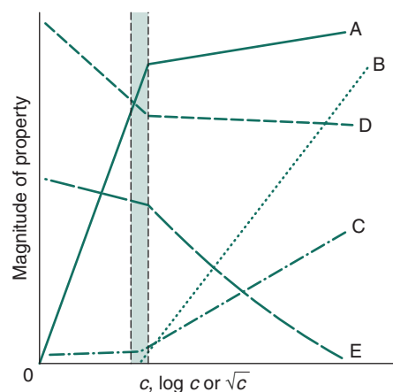
Fig. 5.12 Solution properties of an ionic surfactant as a function of concentration, c : osmotic pressure against c (A); solubility of a water-insoluble solubilize against c (B); intensity of light scattered by the solution against c (C); surface tension against \log c (D); molar conductivity against \sqrt{c} (E).
