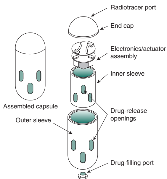
Fig. 21.8 The IntelliSite capsule, with integral electronics/actuator assembly, drug reservoir (0.8 mL) and facility to load with a radioactive marker to allow in situ visualization of the capsule by gamma scintigraphy. (From Wilding, I., Hirst, P., Connor, A., 2000. Development of a new engineering-based capsule for human drug absorption studies. Pharm. Sci. Tech. Today , 3, 385–392, with permission.)
