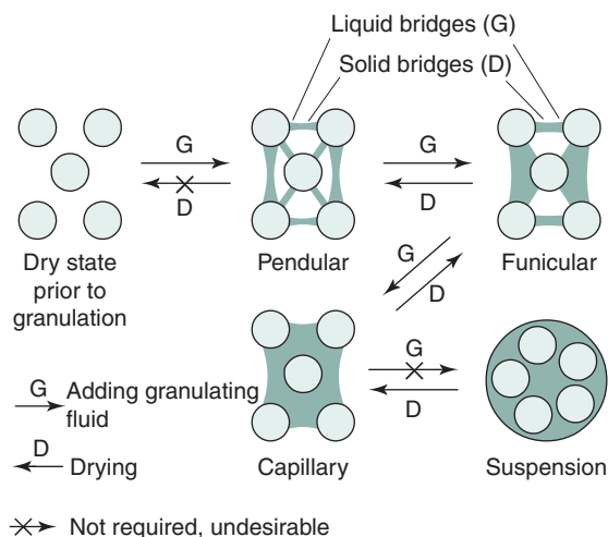
Fig. 29.2 Water distribution between particles of a granule during formation and drying.
