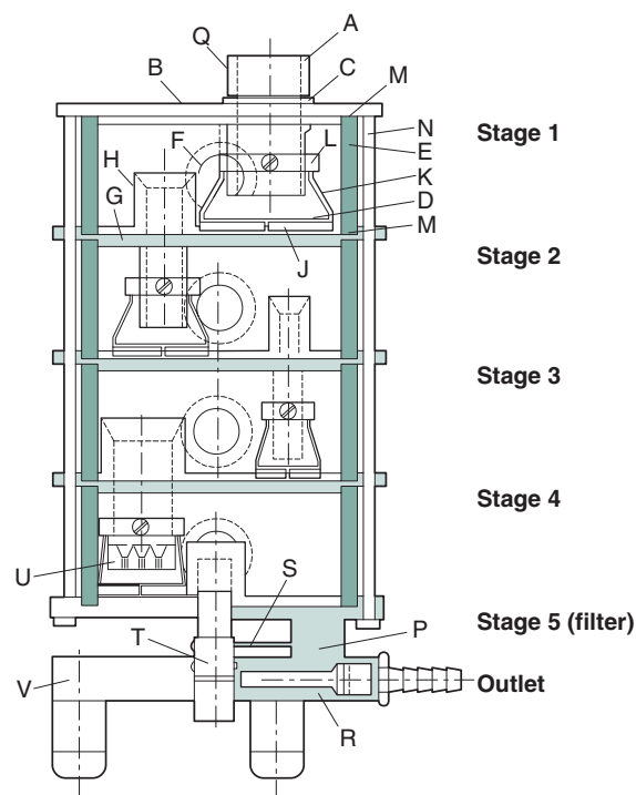
Fig. 39.15 The multistage liquid impinger. (Courtesy of AstraZeneca.)
