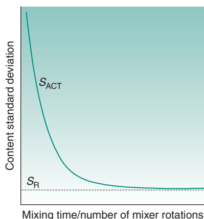
Fig. 11.3 The reduction in content standard deviation as a random mix is approached. S_{ACT} represents the content standard deviation of samples taken from the mix and S_R represents the standard deviation expected from a random mix.
