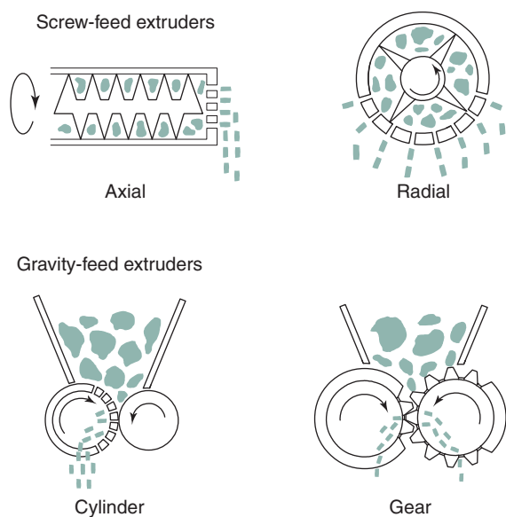
Fig. 29.8 Production extruders.
