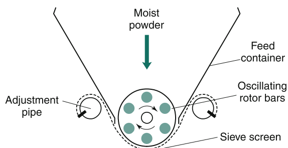
Fig. 29.6 Oscillating granulator.
