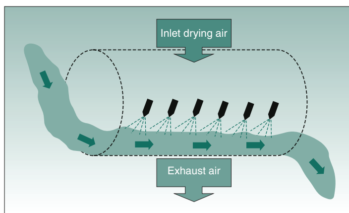
Fig 33.4 Schematic of a continuous coating pan.
