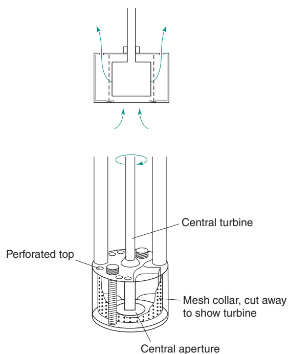
Fig. 11.13 Turbine mixer.
