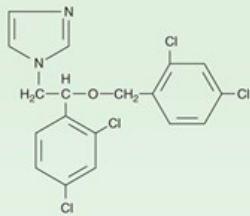
Miconazole
