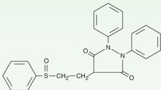
Sulfipyrazone
