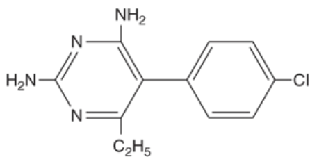
Pyrimethamine
