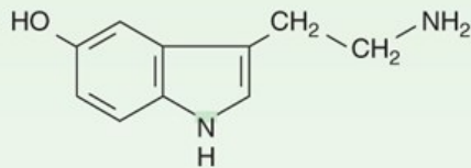
5-Hydroxytryptamine (serotonin)
