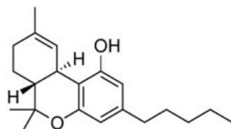
\Delta^9 -Tetrahydrocannabinol
