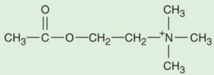
Acetylcholine
