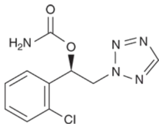
Cenobamate
