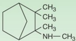
Mecamylamine
