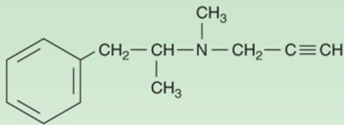
Selegiline
