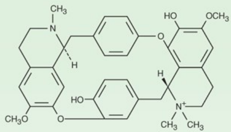
Tubocurarine
