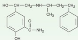
Labetalol
