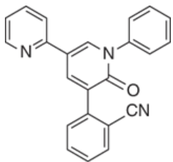
Perampanel
