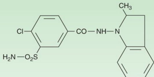
Indapamide
