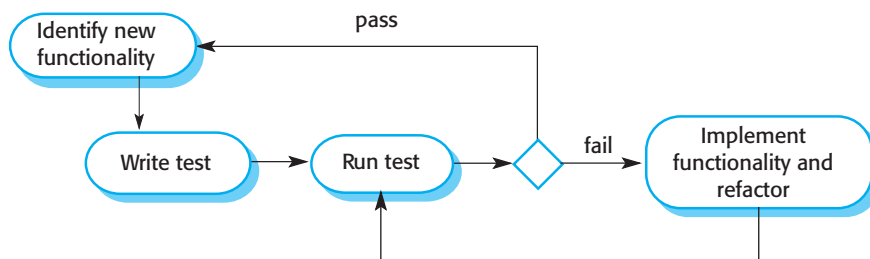
Figure 8.9 Test-driven development
