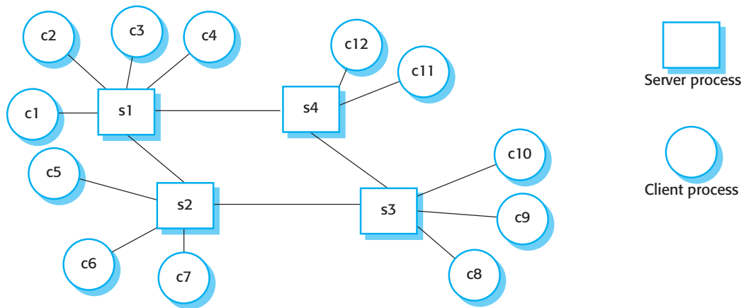
Figure 17.4 Client-server interaction
