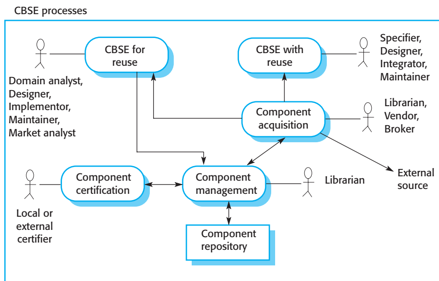
Figure 16.6 CBSE processes
