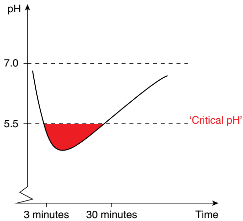
Figure 2.10 Schematic drawing of a Stephan response curve marking the location of the so-called critical pH.
