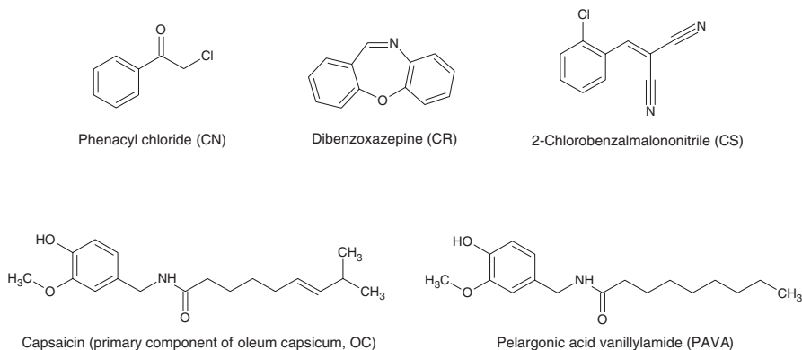
Fig. 6.1 Structures of some chemical crowd control agents
