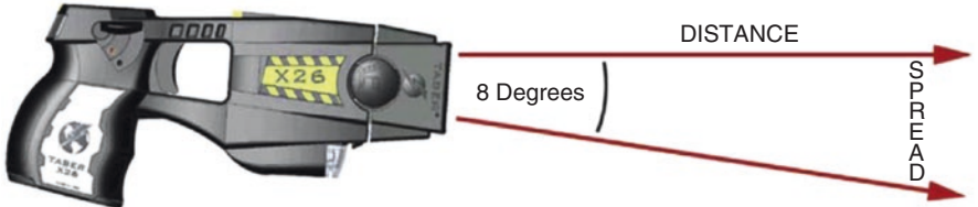
Fig. 8.2 The lower probe of the TASER is launched at an angle of 8° below the laser line
