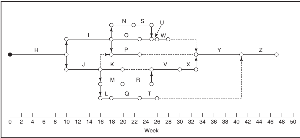
Figure 9.14 Time-based network for the LOGON project using early start times.
