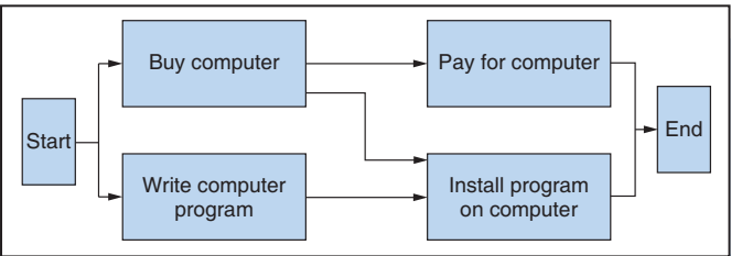
Figure 7.30 AON diagram.
