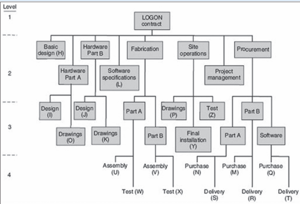
Figure 6.5 Work breakdown structure for the LOGON project. Work packages are lettered H through Z.
