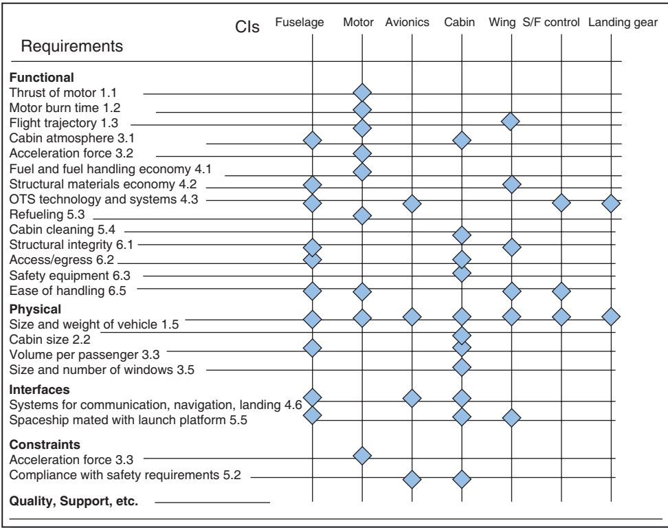
Figure 4.12 Allocation (traceability) matrix.
