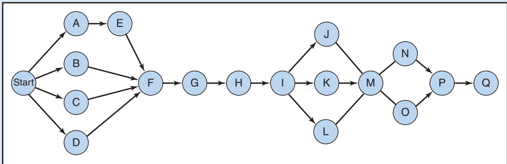
Figure 8.13 Project network.
