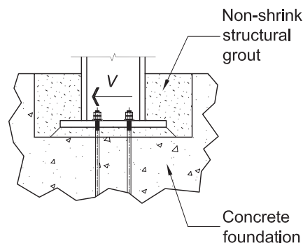
Fig. 4-14. Transfer of base shear through bearing by encasing the column.
