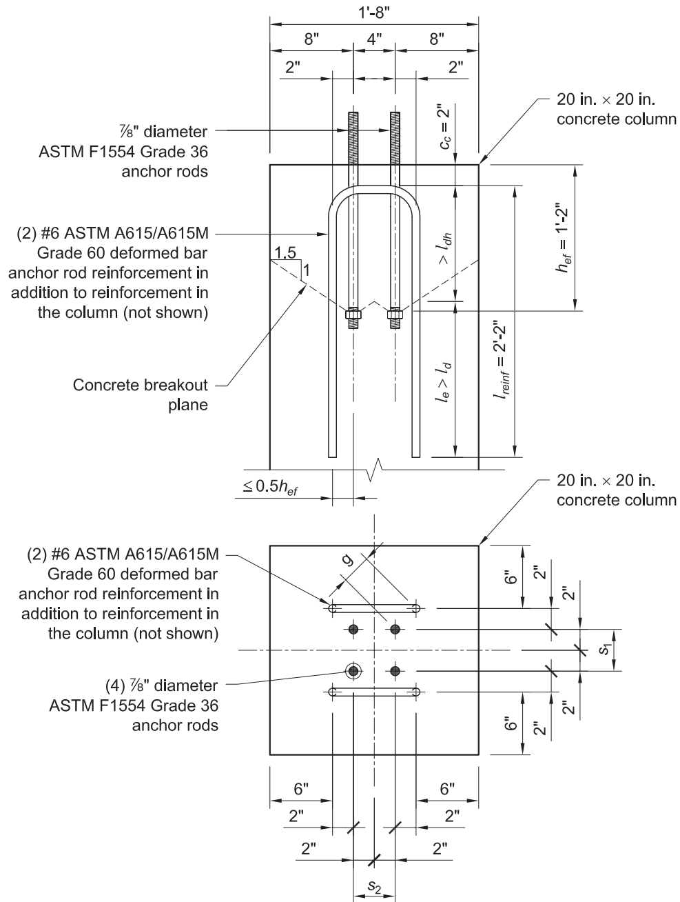
Fig. 4-36. Anchor and reinforcement detailed in Example 4.7-15.
