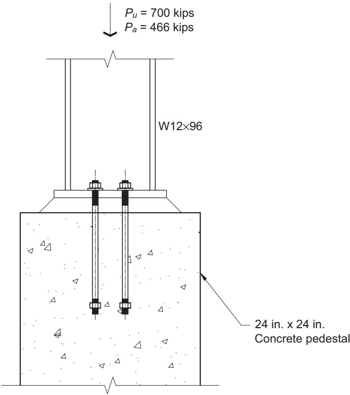
Fig. 4-21. Example 4.7-1 base detail.
