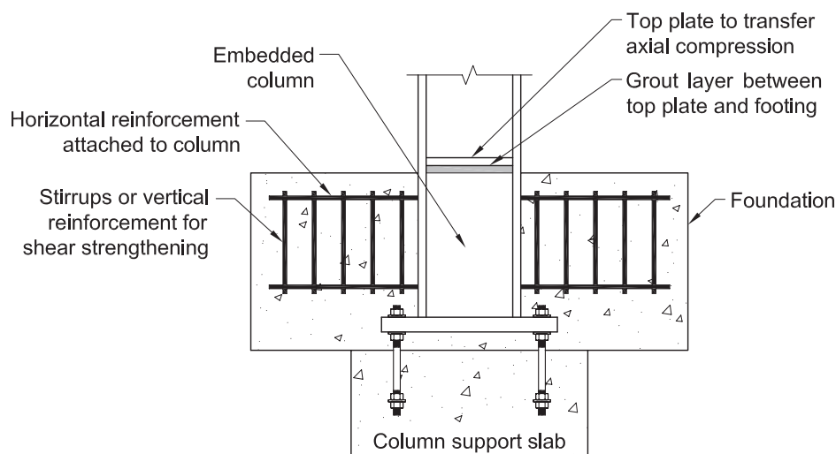
Fig. 5-1. Embedded base connection showing details.
