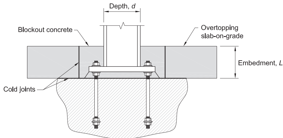
Fig. C-3. Blockout connection with L and D dimensions used for stiffness estimation.
