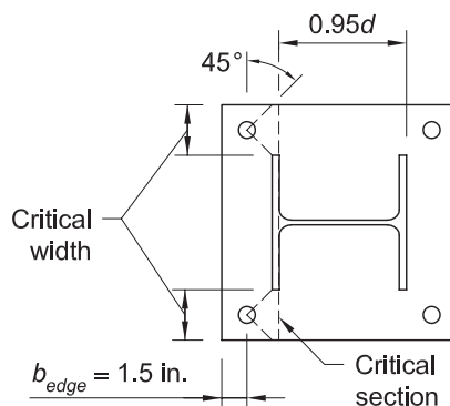
Fig. B-5. Critical plate width for anchor rod (tension side).
