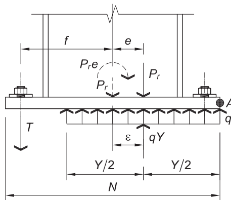
Fig. 4-7. Base plate with low moment.
