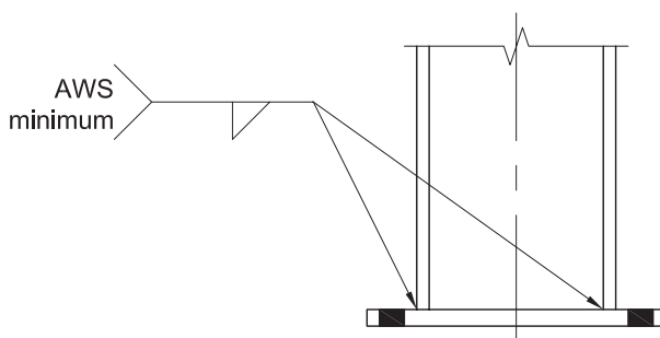
Fig. 4-15. Typical gravity column base plate weld.
