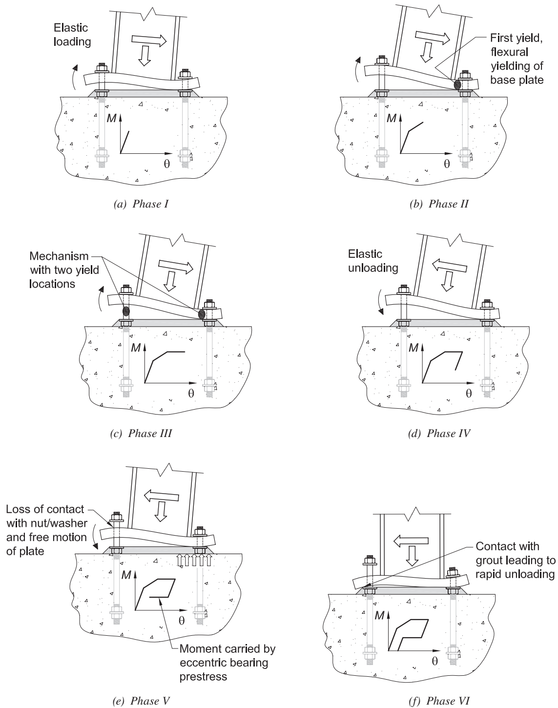
Fig. C-5. Physical phenomena controlling response.
