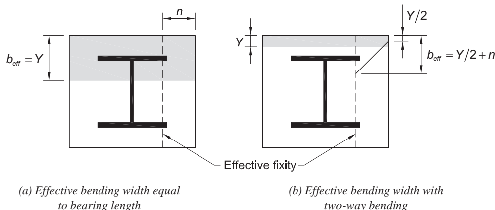
Fig. B-8. Effective width for two-way bending of base plates.
