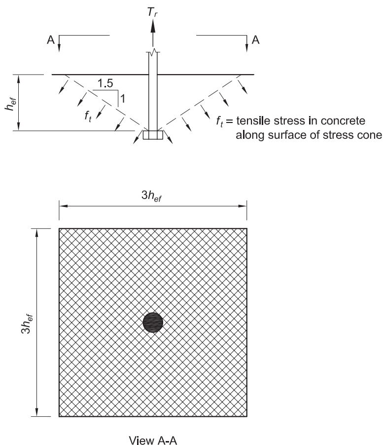
Fig. 4-2. Full breakout cone in tension per ACI 318.
