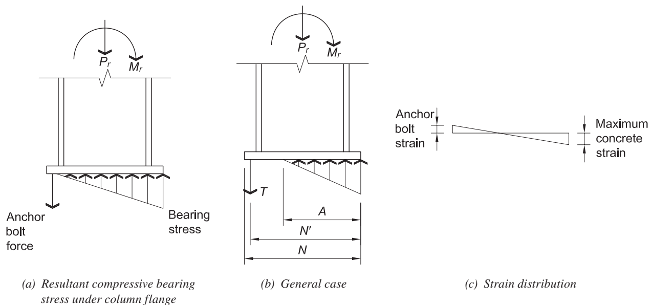
Fig. B-1. Triangular stress distribution for axial load plus moment.
