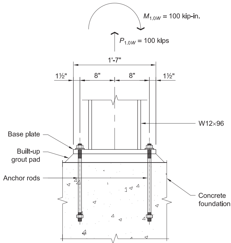
Fig. 4-35. Base configuration and dimensions used in Example 4.7-13.
