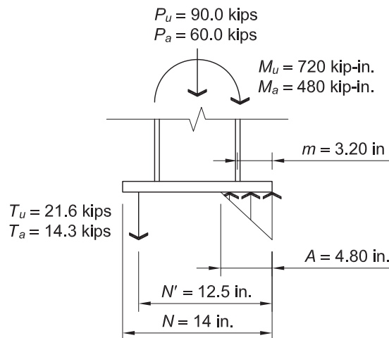
Fig. B-4. Design example with large eccentricity.
