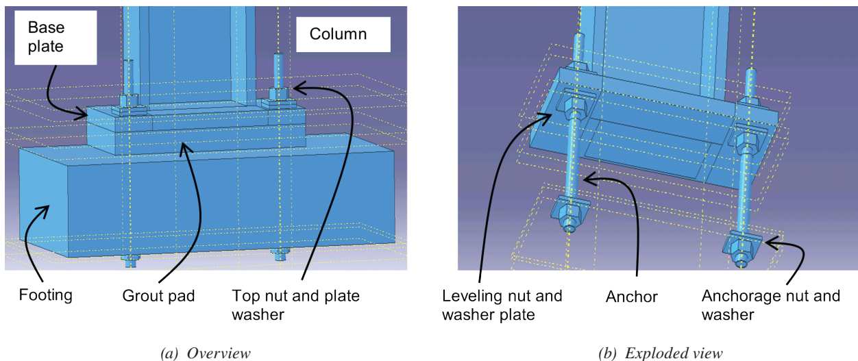
Fig. D-2. Modeled geometry of a base connection.
