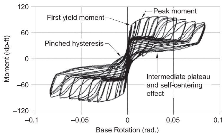
Fig. C-4. Moment rotation response of exposed base plate connection (from Gomez et al., 2010).
