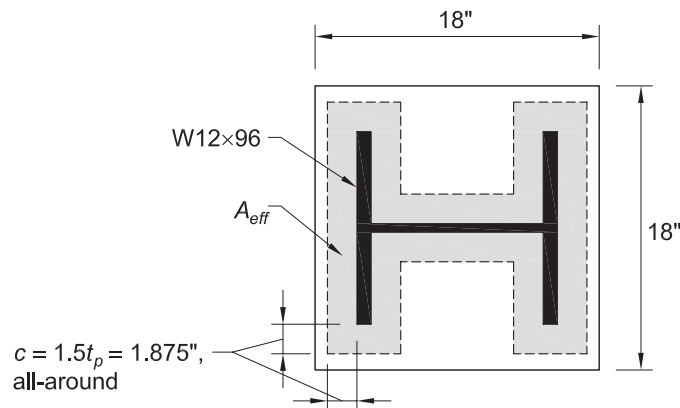
Fig. B-7. Design of base plate under axial compression.
