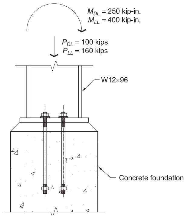
Fig. 4-32. Base detail section as used in Example 4.7-10.
