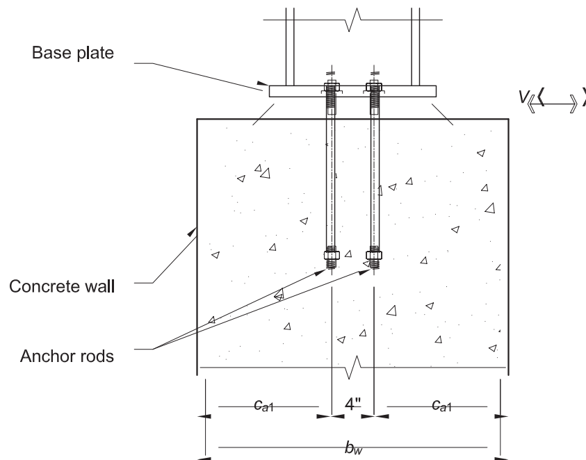
Fig. 4-24. Base connection section for configuration used in Example 4.7-4.
