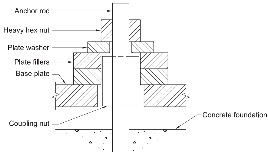
Fig. 4-18. Coupling nut detail for extending anchor rods.
