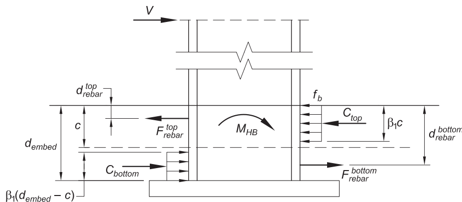
Fig. 5-3. Moment and shear transfer in Type I connections.
