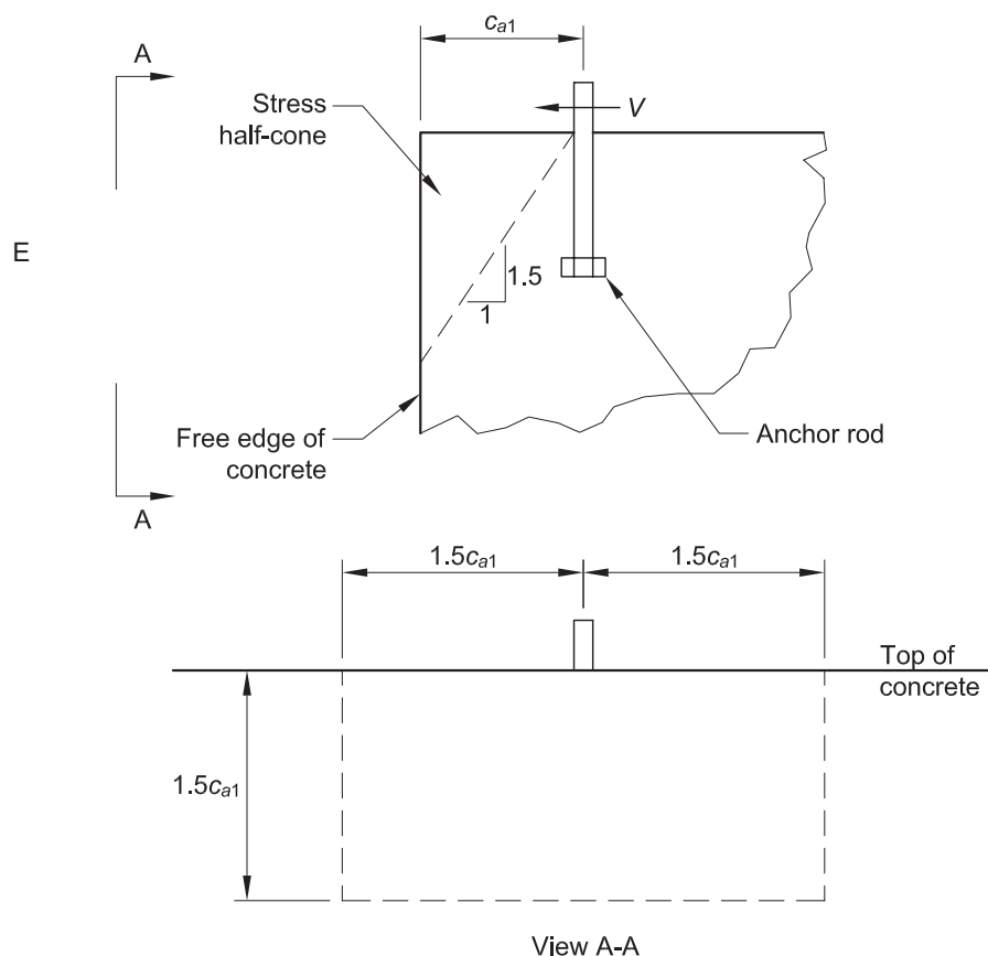
Fig. 4-6. Concrete breakout cone for shear.
