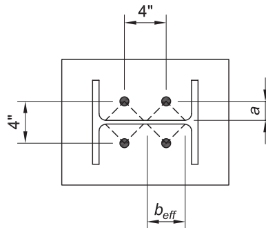
Fig. 4-22. Rod load distribution.
