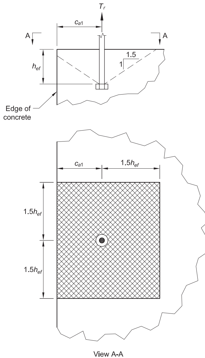
Fig. 4-3. Breakout cone in tension near an edge.
