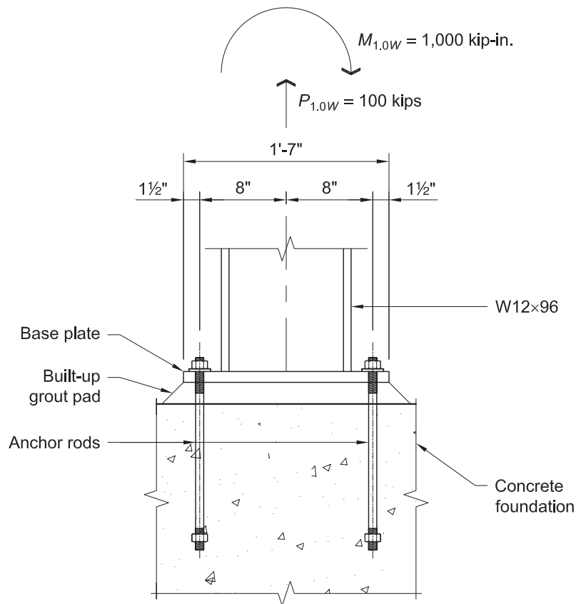
Fig. 4-34. Base connection configuration as detailed in Example 4.7-12.
