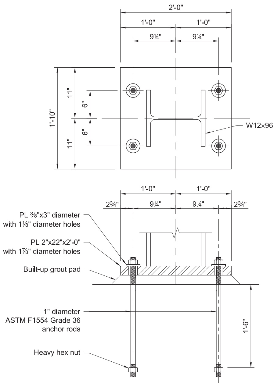
Fig. 4-33. Base connection as detailed in Example 4.7-11.
