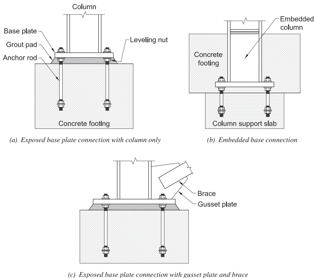
Fig. 1-1. Types of base connections.
