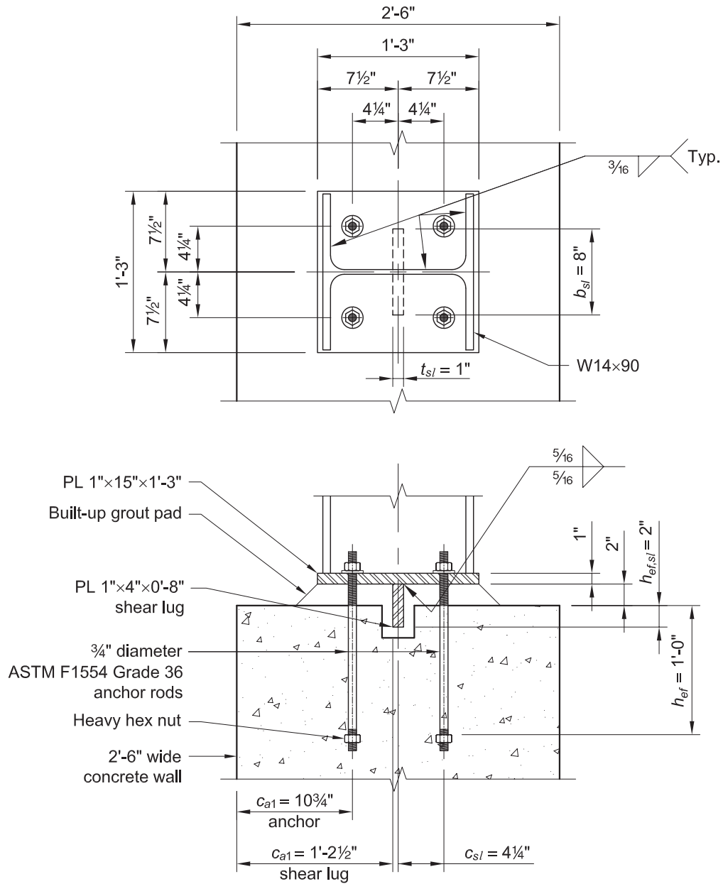
Fig. 4-26. Base connection as detailed in Example 4.7-5.
