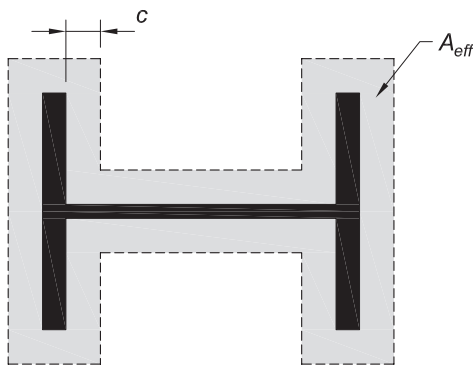
Fig. B-6. Effective bearing area to account for plate flexibility.
