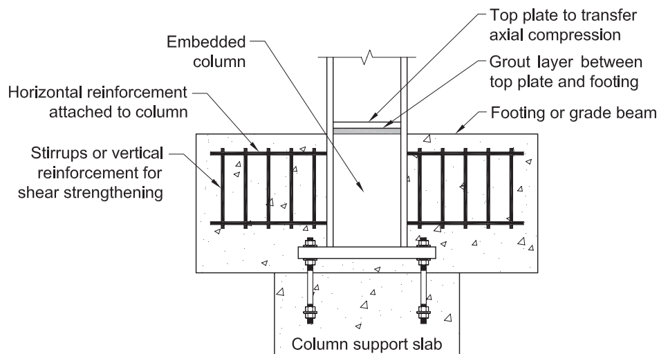
Fig. 3-4. Embedded base connection showing details.
