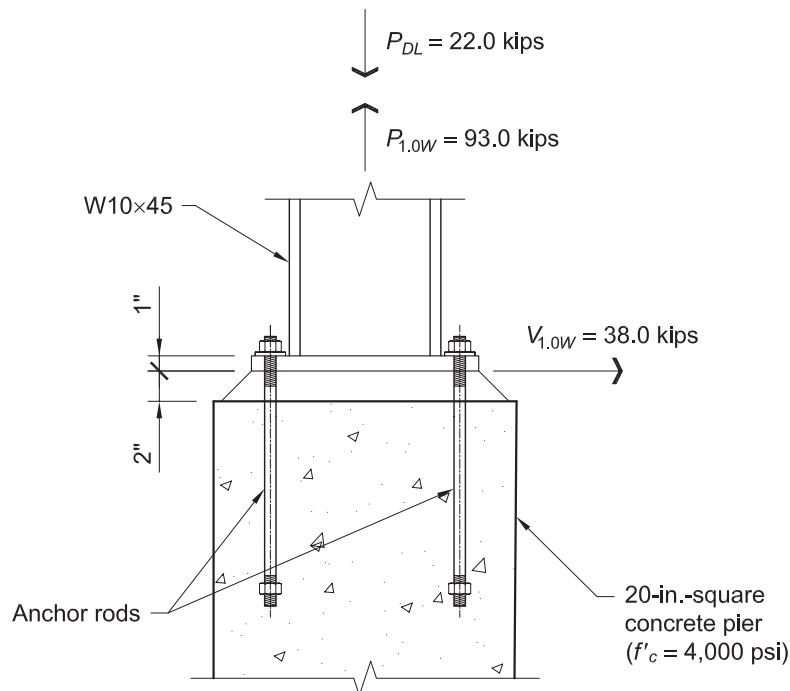
Fig. 4-27. Applied loading and base connection configuration used in Example 4.7-6.
