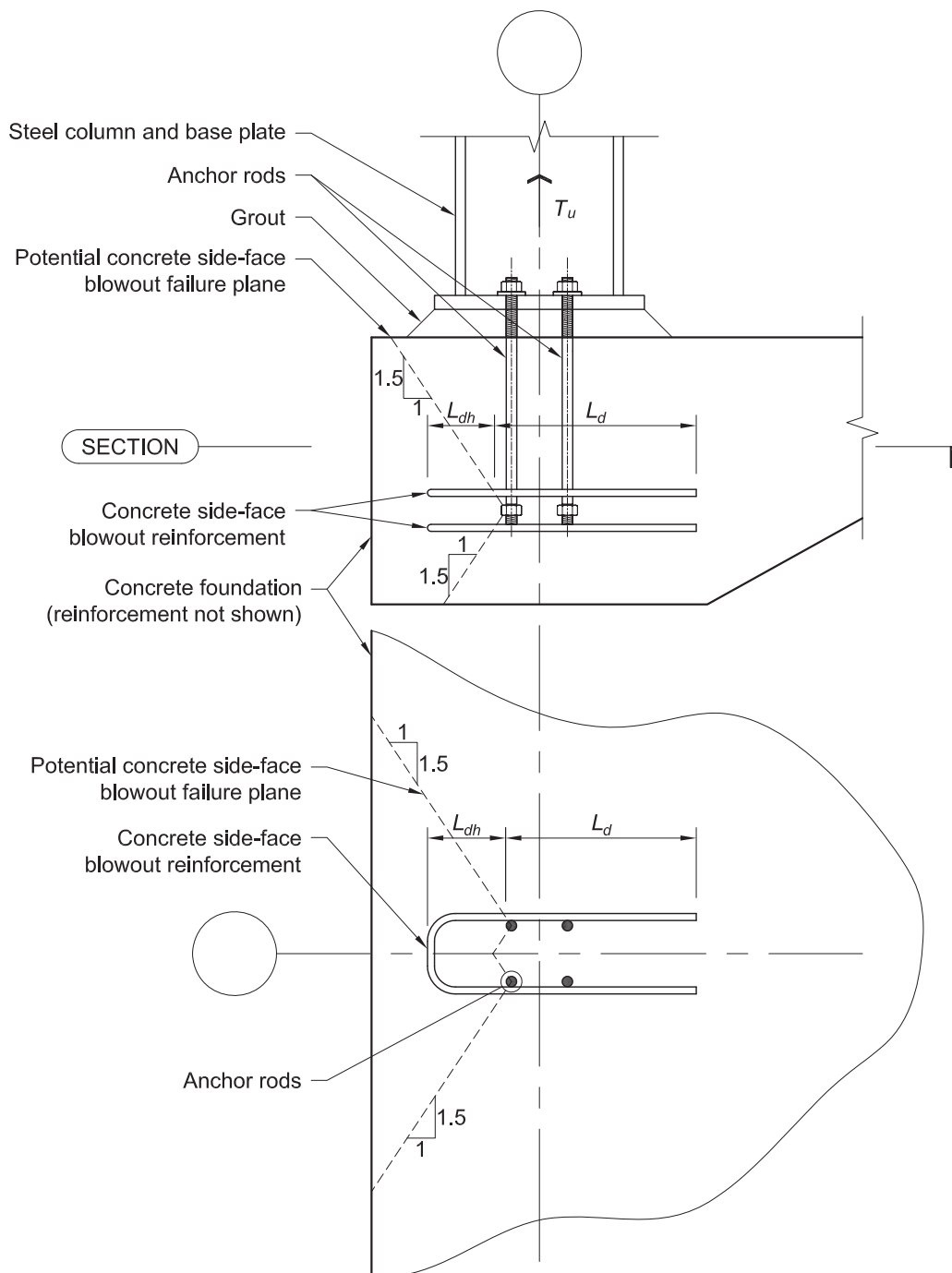
Fig. 4-13. The use of steel reinforcement for restraining concrete side-face blowout.
