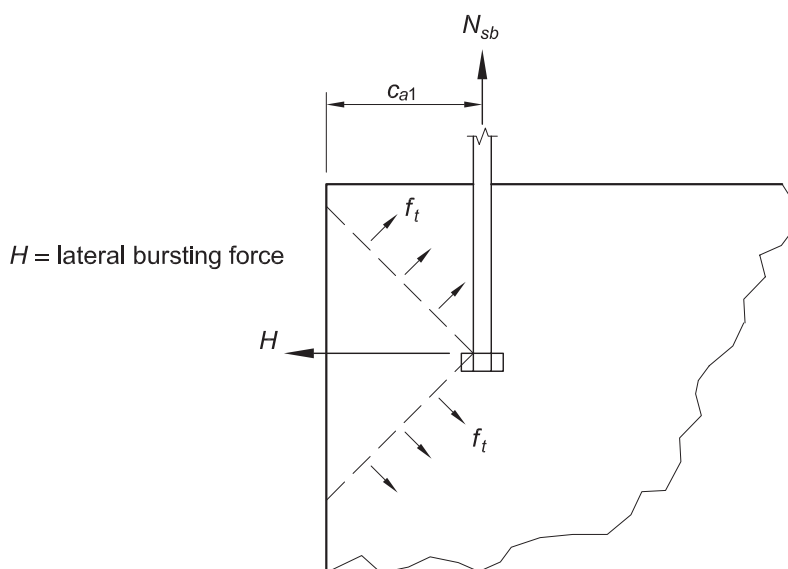
Fig. 4-4. Lateral bursting forces for anchor rods in tension near an edge.
