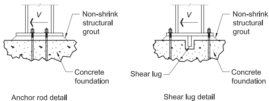
Fig. 4-5. Transfer of base shear.
