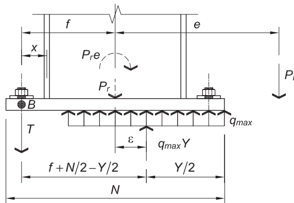
Fig. 4-8. Base plate with large moment.
