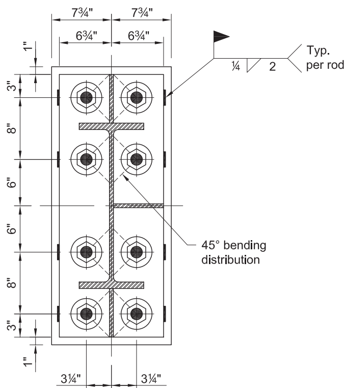
Fig. 4-29. Base connection plan view as detailed in Example 4.7-7.
