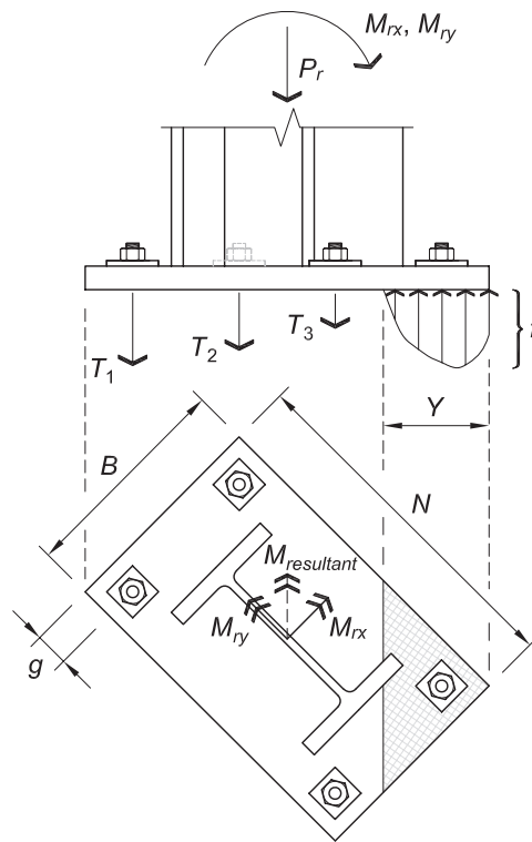
Fig. 4-10. Base plate subjected to biaxial bending resulting in static indeterminacy.
