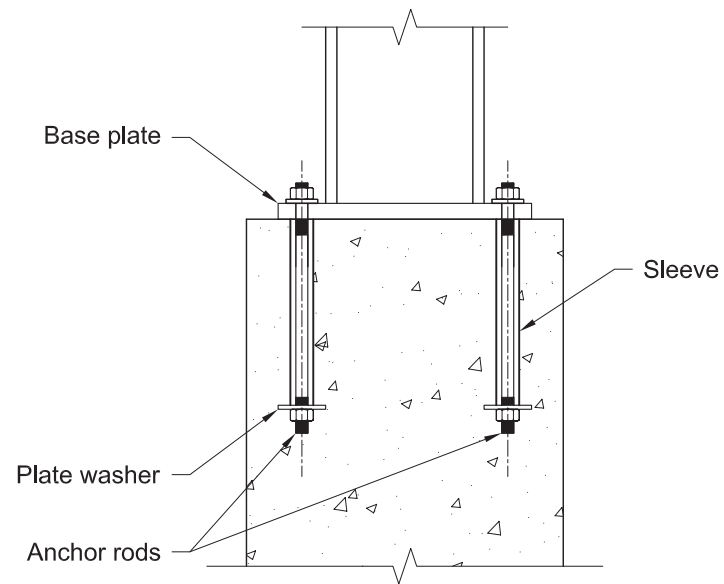
Fig. A-1. Anchor rods with sleeves.
