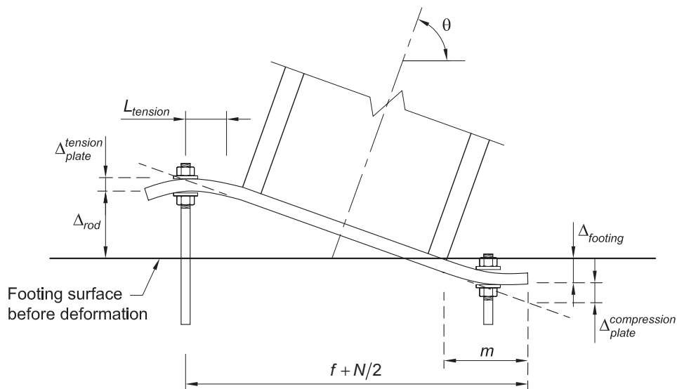
Fig. C-2. Contributors to deformation of exposed base plate connection.
