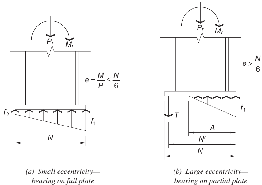
Fig. B-2. Effect of eccentricity on bearing.
