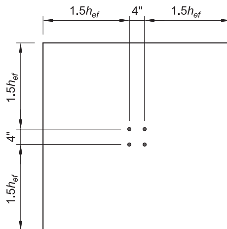
Fig. 4-23. Breakout cone for Example 4.7-3.
