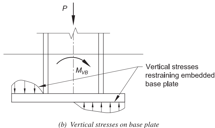
Fig. 5-5. Load transfer in Type II connections.
