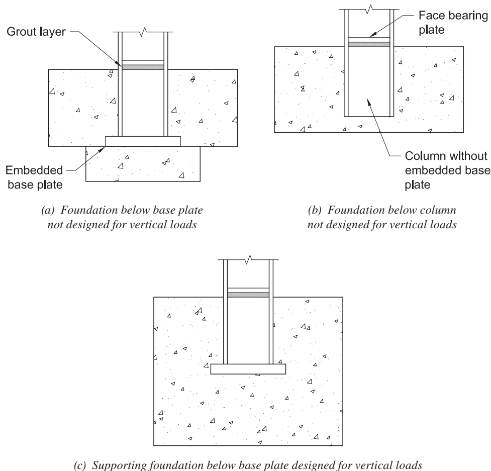
Fig. 5-2. Embedded column base connection configurations.
