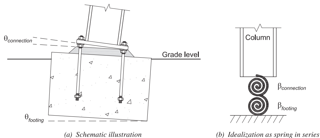
Fig. C-1. Deformation at column base.
