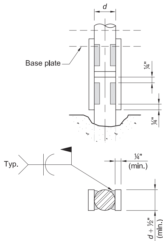
Fig. 4-20. Lap plate splice.
