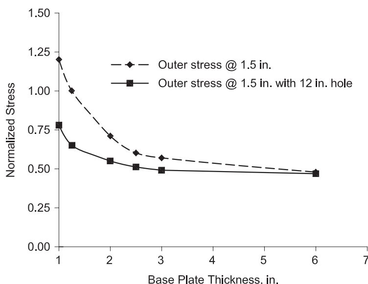
Fig. A-3. Stresses in base plate.
