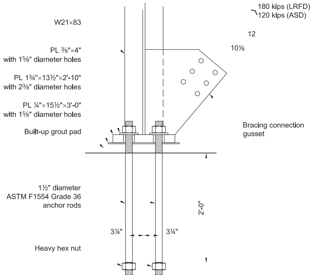
Fig. 4-28. Base connection as detailed in Example 4.7-7.
