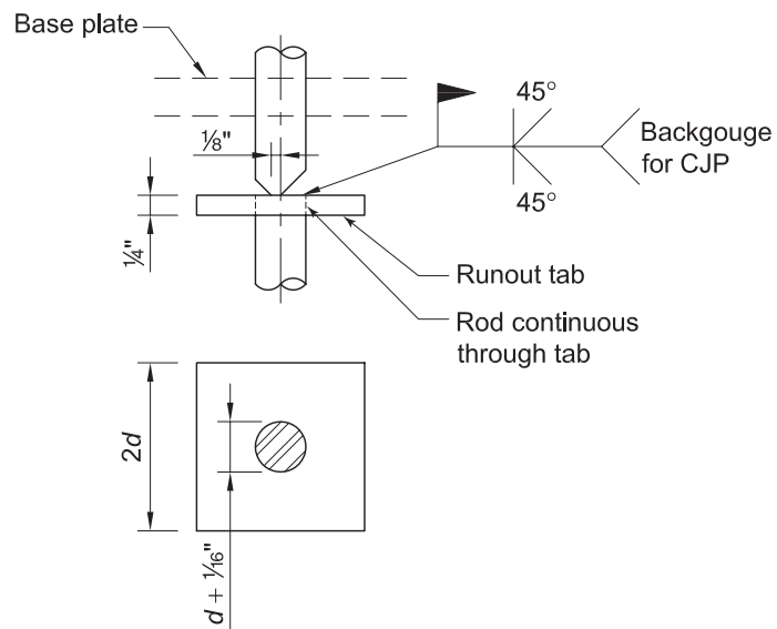
Fig. 4-19. Groove weld splice.
