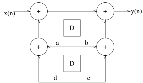
Direct form II :
