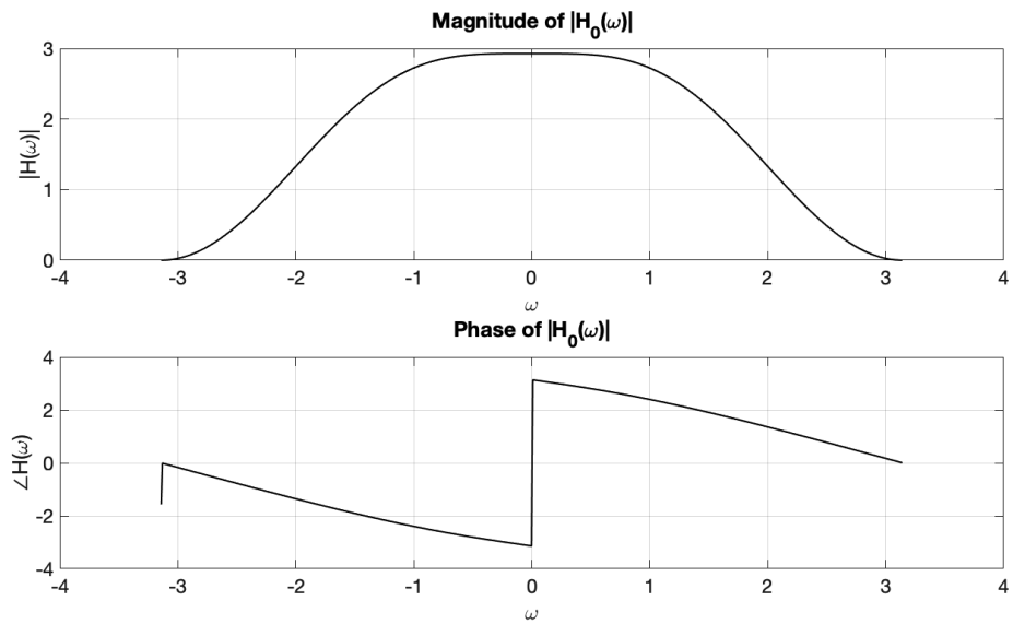
Figure 12.16-1: Magnitude and phase of H_0(\omega)
