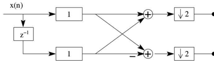
Figure 12.4-1: Analysis section
