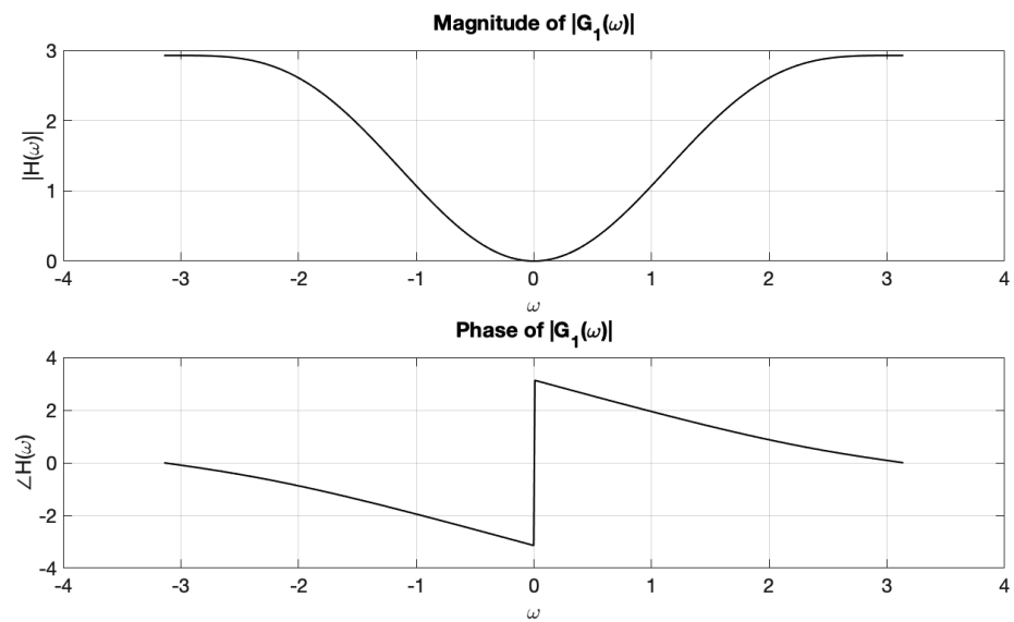
Figure 12.16-4: Magnitude and phase of G_1(\omega)
