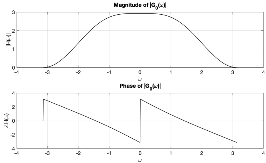
Figure 12.16-3: Magnitude and phase of G_0(\omega)
