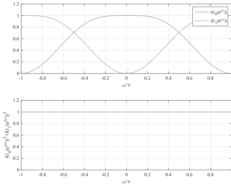
Figure 12.33-7: Frequency responses of the Daubechies DB4 or db2 filters and verification that they satisfy the perfect reconstruction condition.
