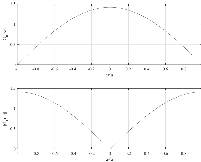
Figure 12.26-6: Magnitude frequency responses of the scaling and wavelet Haar filters.
