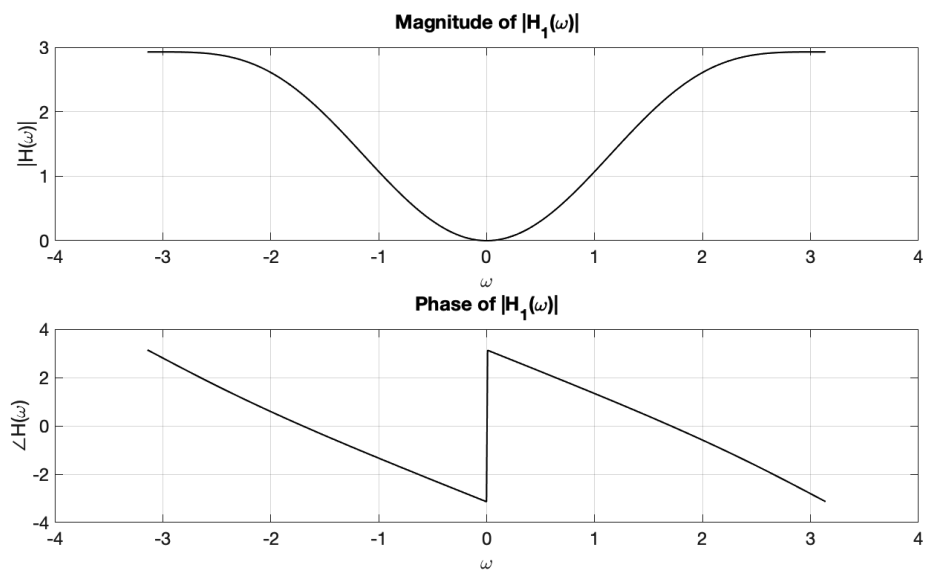
Figure 12.16-2: Magnitude and phase of H_1(\omega)
