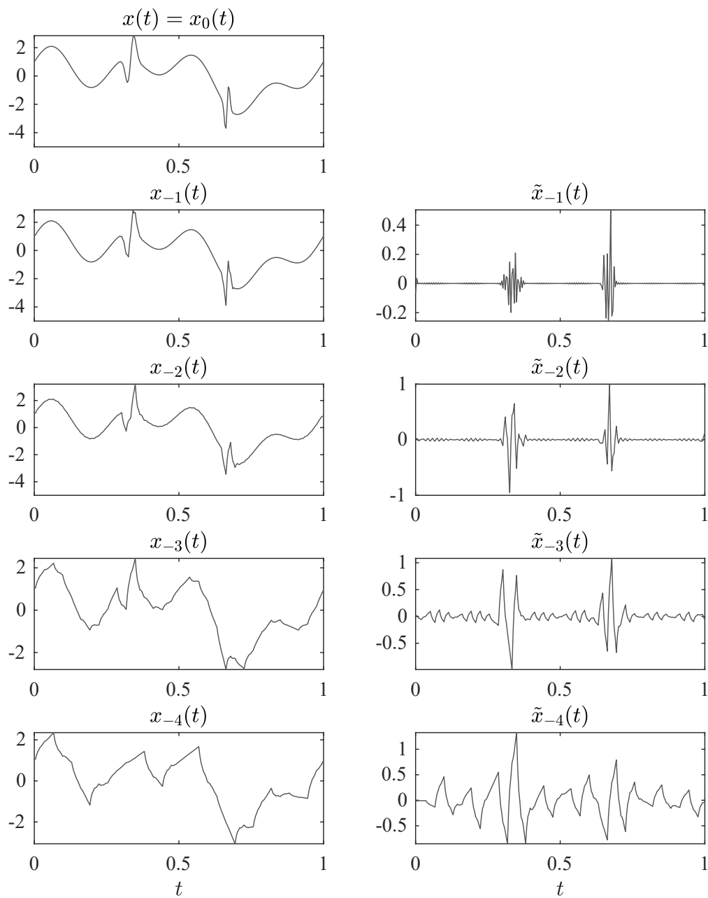
Figure 12.34-8: Decomposition using the db2 Daubechies wavelet with N = 4 .
