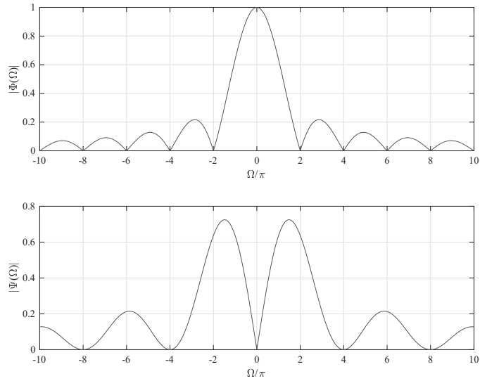
Figure 12.24-5: Spectra of the scaling and wavelet Haar functions.
