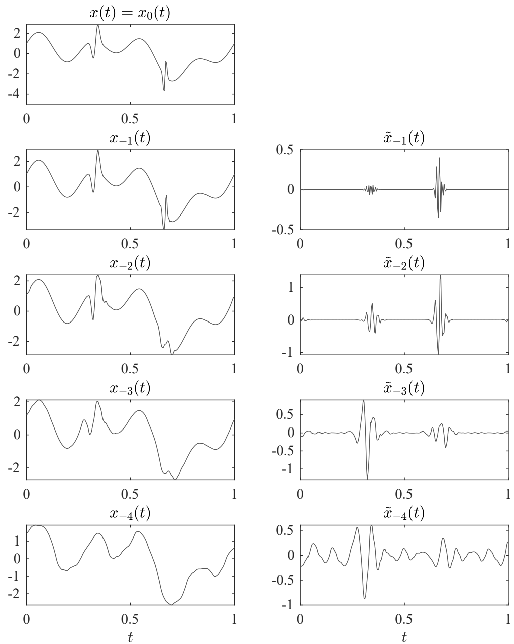
Figure 12.34-9: Decomposition using the db4 Daubechies wavelet with N = 8 .
