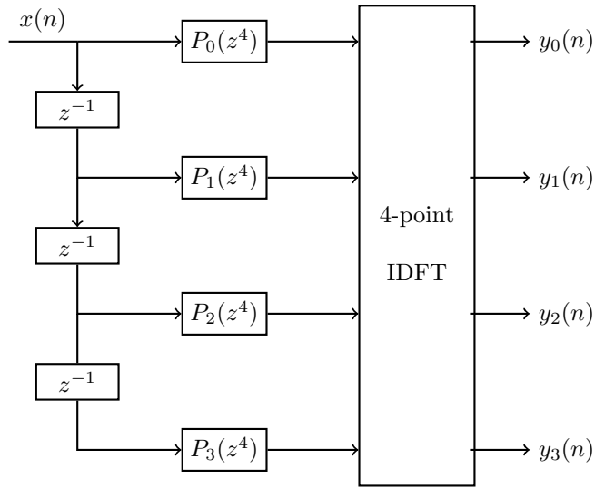
Figure 12.2-1: Analysis section of the DFT filter bank
