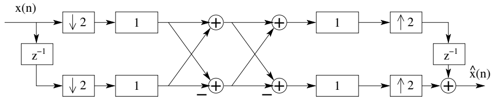
Figure 12.4-2: QMF in a polyphase realization
