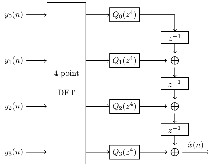
Figure 12.2-2: Synthesis section of the DFT filter bank
