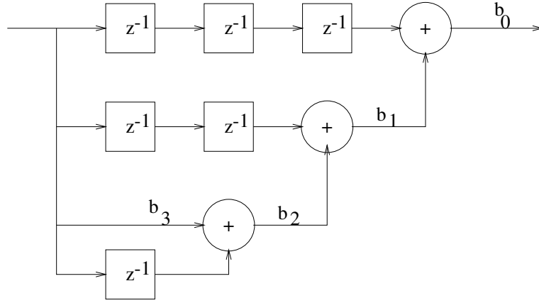
Figure 9.26-2: Structure of H(z) = b_0 z^{-3} + b_0 b_1 z^{-2} + b_0 b_1 b_2 z^{-1} + b_0 b_1 b_2 b_3
