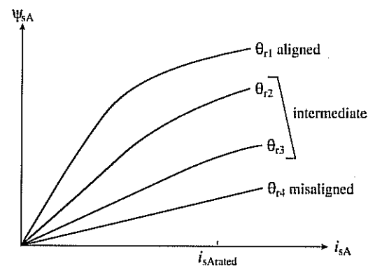
Fig. 5.3. Flux linkage versus stator current for various rotor positions.
