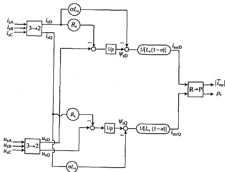
Fig. 4.9(a). Flux model in the stationary reference frame (the inputs are u_{sA}, u_{sB}, u_{sC}, i_{sA}, i_{sB}, i_{sC} ).
