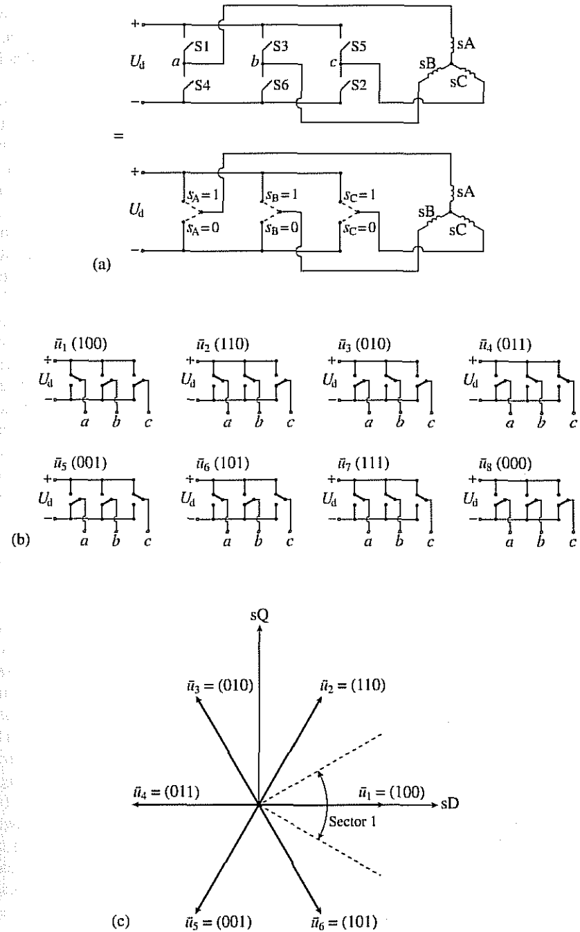
Fig. 4.83. Schematic of PWM VSI inverter, the eight switching states and the corresponding switching space vectors. (a) PWM VSI; (b) switching stages; (c) switching-voltage space vectors.
