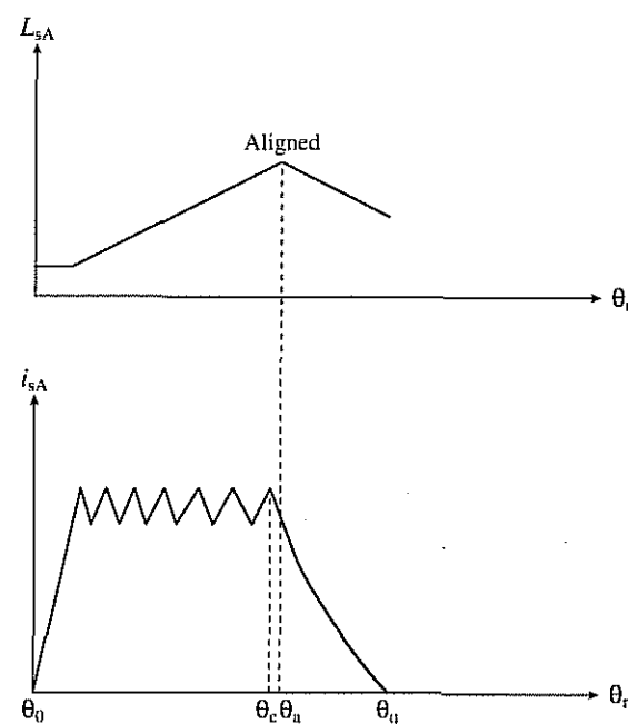
Fig. 5.6. SRM chopping waveforms.
