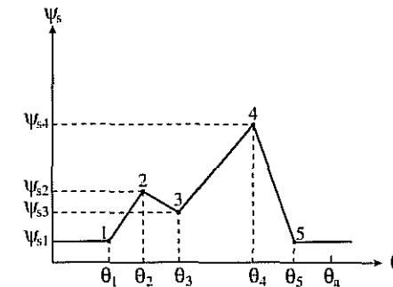
Fig. 5.8. Stator flux reference as a function of rotor position.
