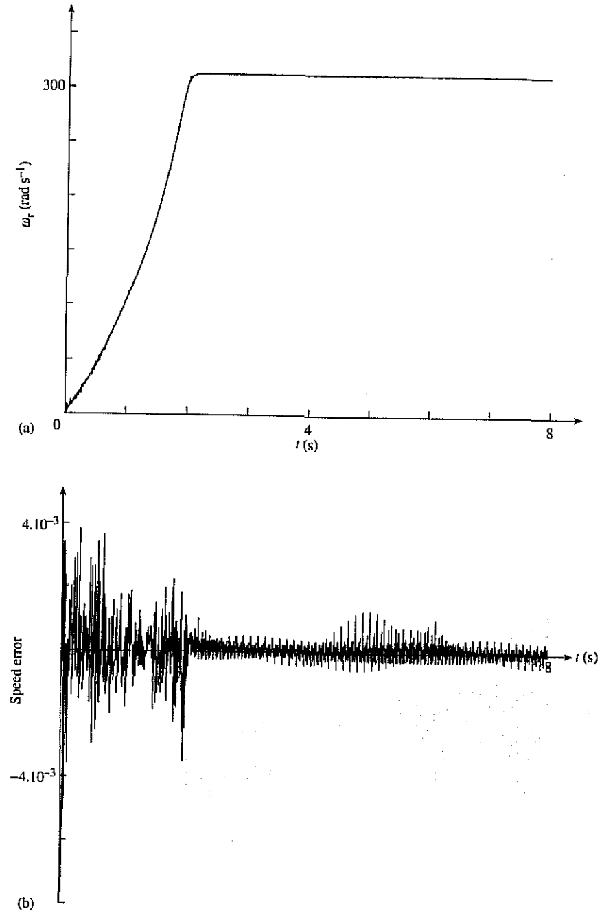
Fig. 7.15. Speed of unloaded squirrel-cage machine during run-up. (a) Speed estimation by 8-9-7-1 ANN; (b) speed error.
