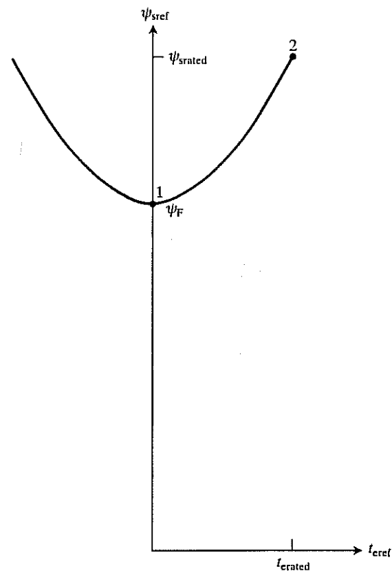
Fig. 3.13. The characteristics implemented by the function generator FG1.
