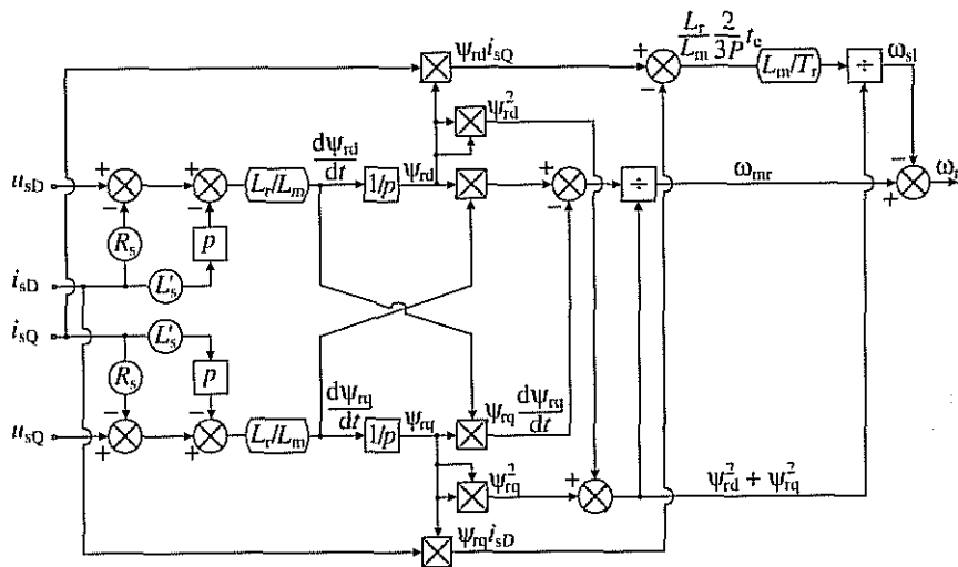
Fig. 4.53. Rotor speed estimator using 2 integrators, 2 differentiators, and 3 parameters.
