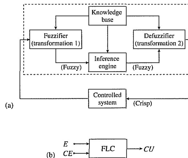
Fig. 4.38. Mamdani type of fuzzy-logic controller (FLC). (a) Schematic block diagram of a control system containing a Mamdani-type of FLC; (b) FLC with two inputs.
