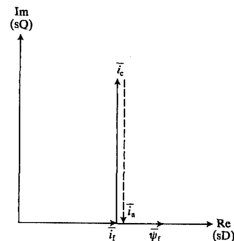
Fig. 2.6. The space phasors in a d.c. machine.
