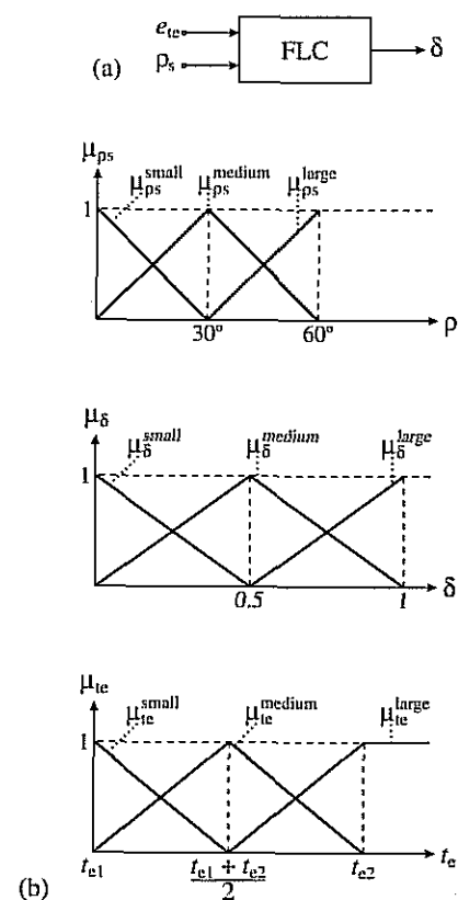
Fig. 4.88. Fuzzy-logic duty-ratio estimator, and membership functions. (a) FLC duty-ratio estimator; (b) membership functions.
