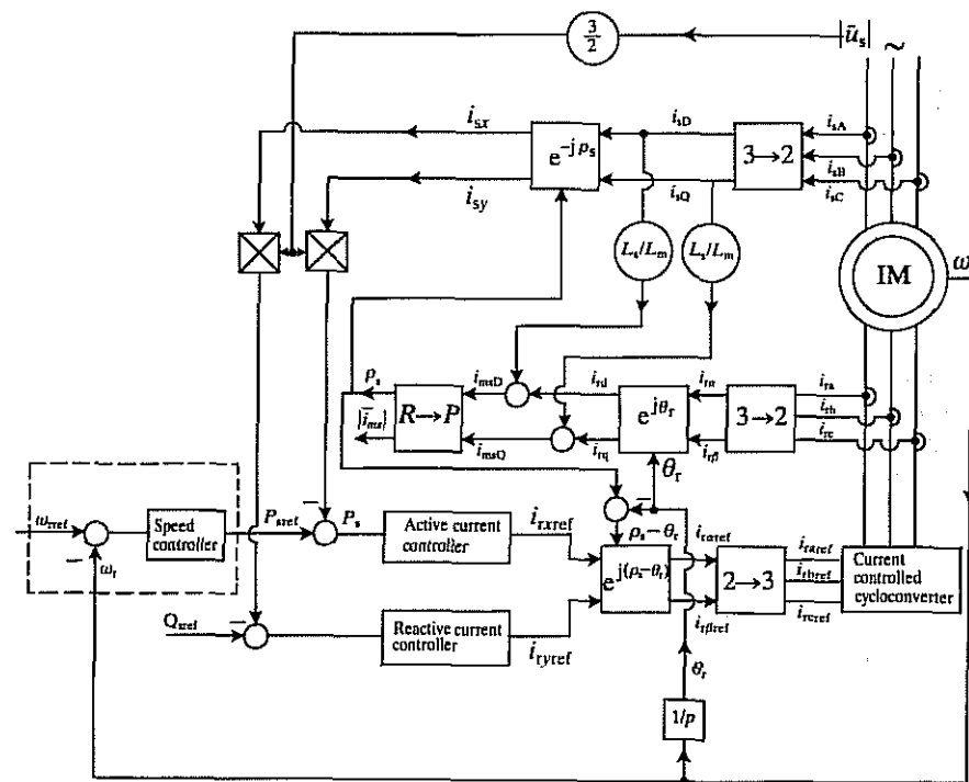
Fig. 4.30. Schematic of the stator-flux-oriented control of a doubly-fed induction machine with a current-controlled cycloconverter in the rotor.
