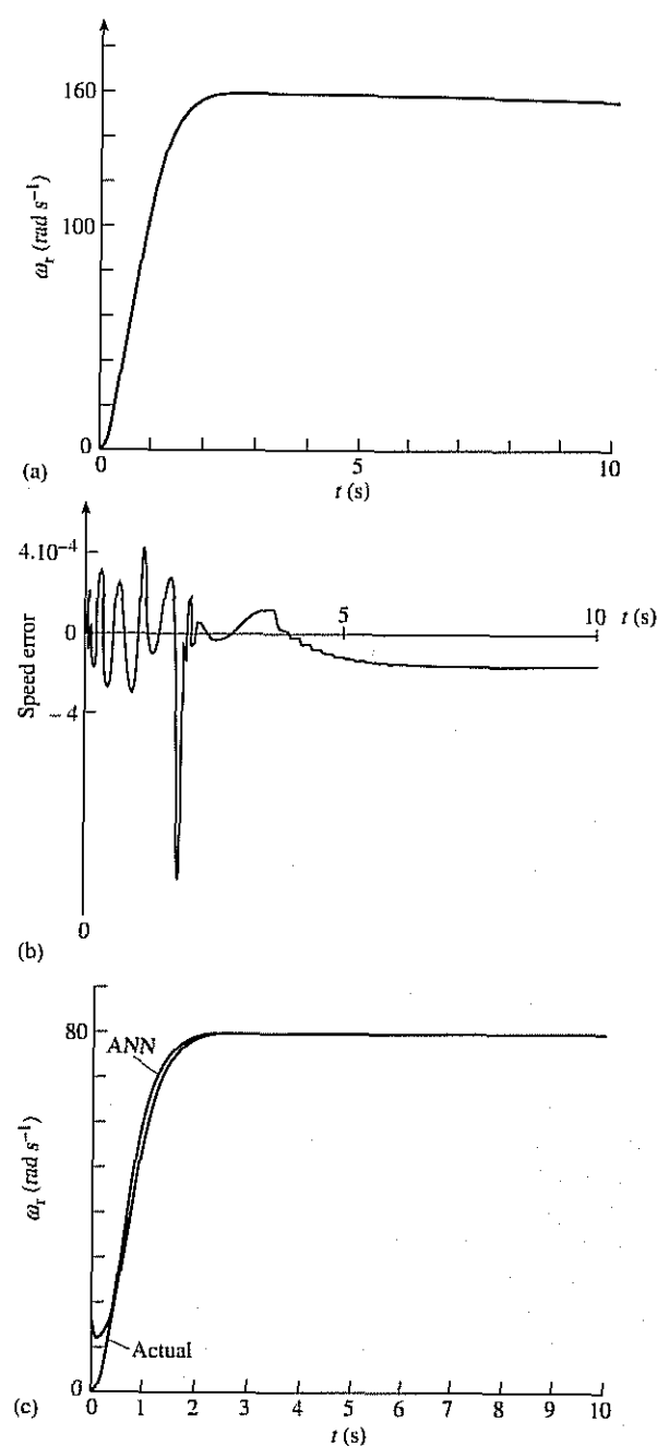
Fig. 7.3. Speed of d.c. machine. (a) Speed obtained by 3-4-2-1 ANN (armature voltage 240 V); (b) speed error; (c) actual speed and speed obtained by ANN (training with sinusoidal armature voltage, checking with constant armature voltage, 120 V).
