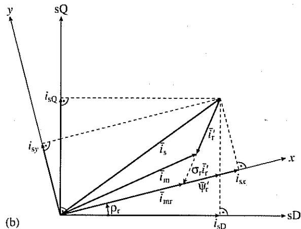
Fig. 1.1. Direct rotor-flux-oriented control of induction motor with impressed stator currents. (a) Drive scheme; (b) vector diagram.
