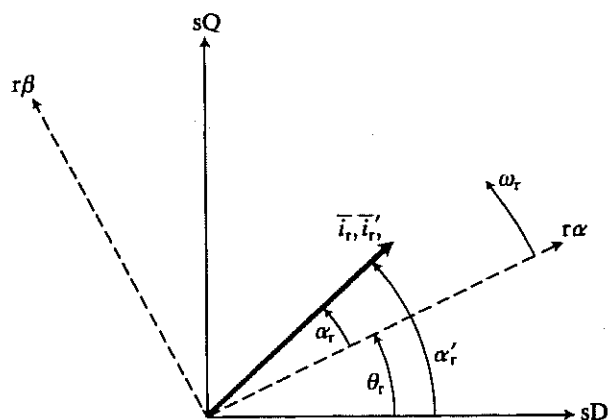
Fig. 2.3. The relationship between the stationary and rotating reference frames.
