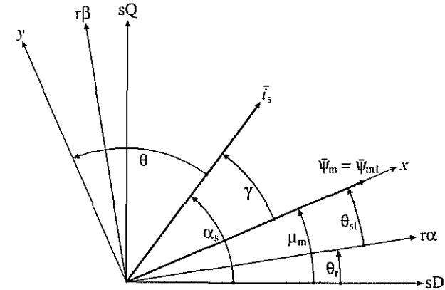
Fig. 4.65. Magnetizing flux-linkage and stator-current space vectors and the various angles.
