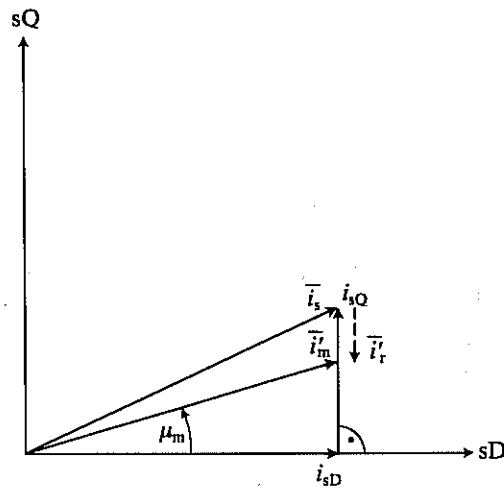
Fig. 2.13. Space phasors of \bar{i}_s , \bar{i}'_r , and \bar{\psi}'_m at instant t > t_0 .
