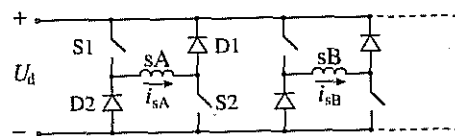
Fig. 5.4. Asymmetrical half-bridge converter.
