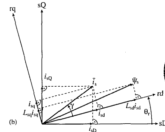
Fig. 1.4. Rotor-oriented control of synchronous reluctance motor supplied by a current-controlled PWM inverter. (a) Drive scheme; (b) vector diagram.
