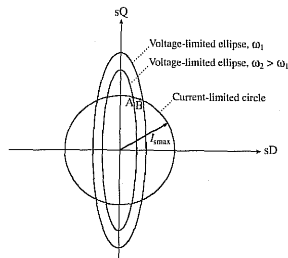
Fig. 6.4. Voltage and current limits in the field-weakening region.
