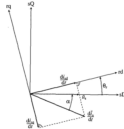
Fig. 3.46. Rate of change of stator-current space vector for a test voltage space vector (at standstill).
