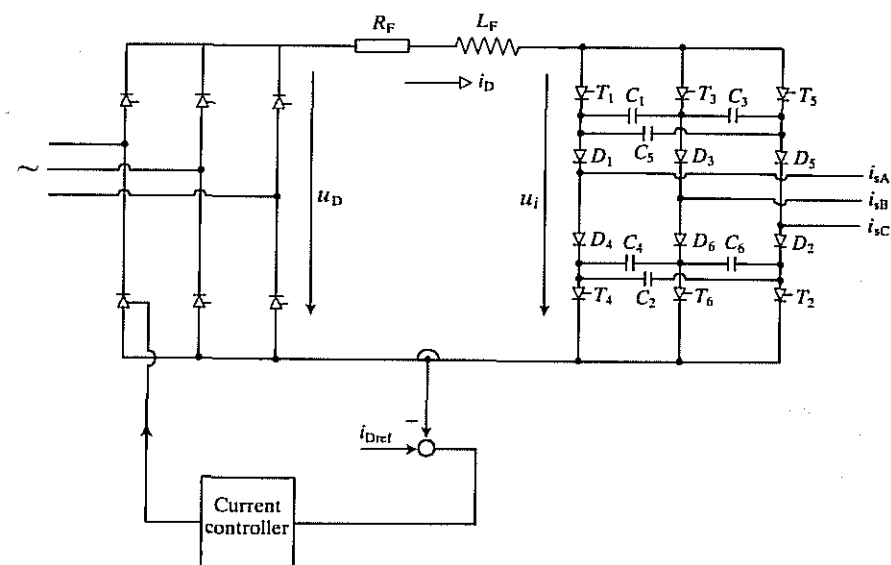
Fig. 4.17. Schematic of conventional six-step CSI with auto-sequential commutation.
