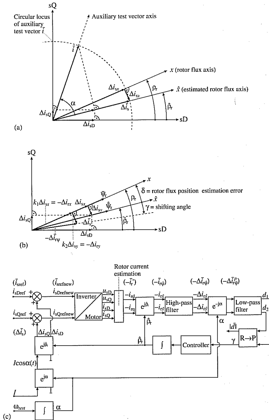
Fig. 4.68. Estimation of rotor flux angle at zero and low frequencies. (a) Vector diagram, production of test vector; (b) vector diagram, effect of saturation on rotor currents; (c) basic estimation scheme.
