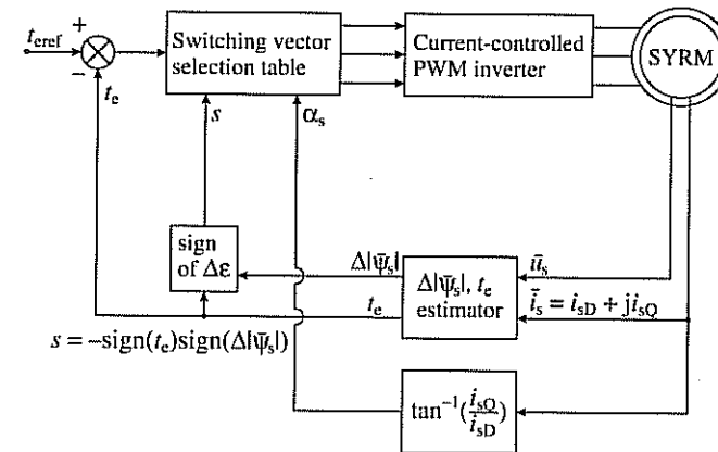
Fig. 3.54. Modified direct-torque-control scheme.
