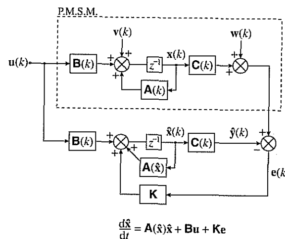
Fig. 3.36. Structure of the EKF.
