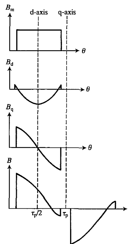
Fig. 3.9. Component and resultant flux-density distributions in the IPM synchronous machine.
