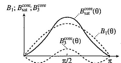
Fig. 4.58. Fundamental, third-harmonic, and peaked flux-density distributions for core saturation.
