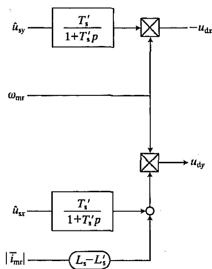
Fig. 4.2. Decoupling circuit to obtain decoupling voltages u_{dx} , u_{dy} (if |\bar{i}_{mr}| = \text{constant} ). Inputs are \hat{u}_{sx} , \hat{u}_{sy} , \omega_{mr} , |\bar{i}_{mr}| .
