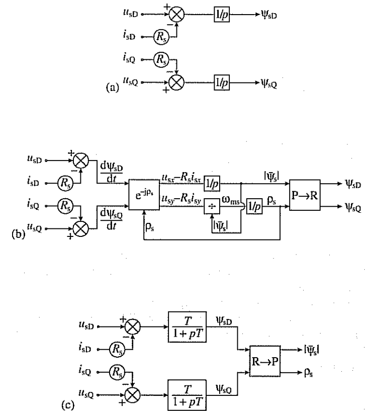
Fig. 3.20. Stator flux-linkage estimators. (a) Estimation in the stationary reference frame; (b) estimation in the stator-flux-oriented reference frame; (c) estimation in the stationary reference frame using quasi-integrators.
