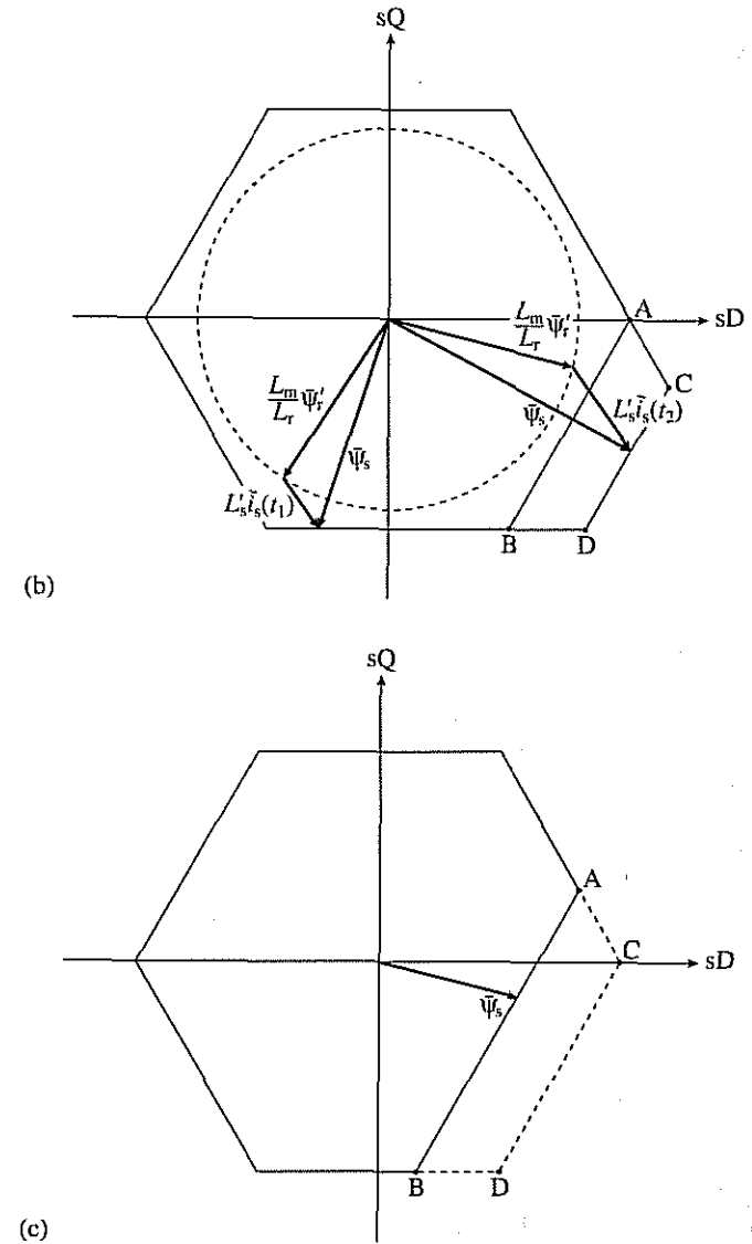
Fig. 4.89. Field-weakening operation: phase retard and phase advance of stator flux-linkage space vector. (a) Phase retard (torque reduction) by applying stop pulse; (b) phase retard (torque reduction) by increasing peripheral length of hexagon around a corner; (c) phase advance (torque increase) by decreasing peripheral length of a hexagon side.
