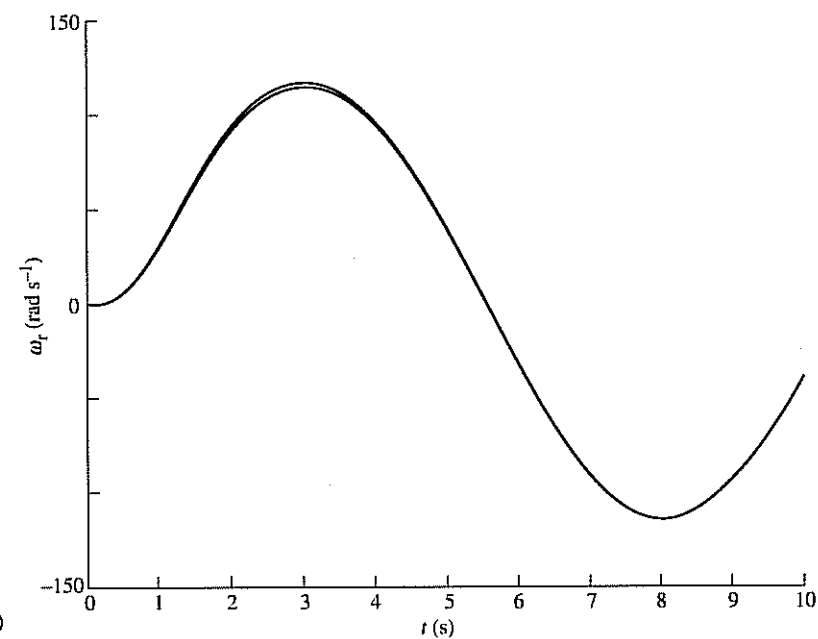
Fig. 7.4. Speed of d.c. machine. (a) Speed obtained by 4-4-2-1 ANN (training with triangular armature voltage, amplitude = 240 V, checking with triangular armature voltage, amplitude = 300 V). (b) Speed obtained by 4-4-2-1 ANN (training with sinusoidal armature voltage, amplitude = 240 V, checking with sinusoidal armature voltage, amplitude = 180 V). (c) Speed obtained by 4-1-1 ANN (training with sinusoidal armature voltage, amplitude = 240 V, checking with sinusoidal armature voltage, amplitude = 180 V). (d) Speed obtained by 4-2-1 ANN.
