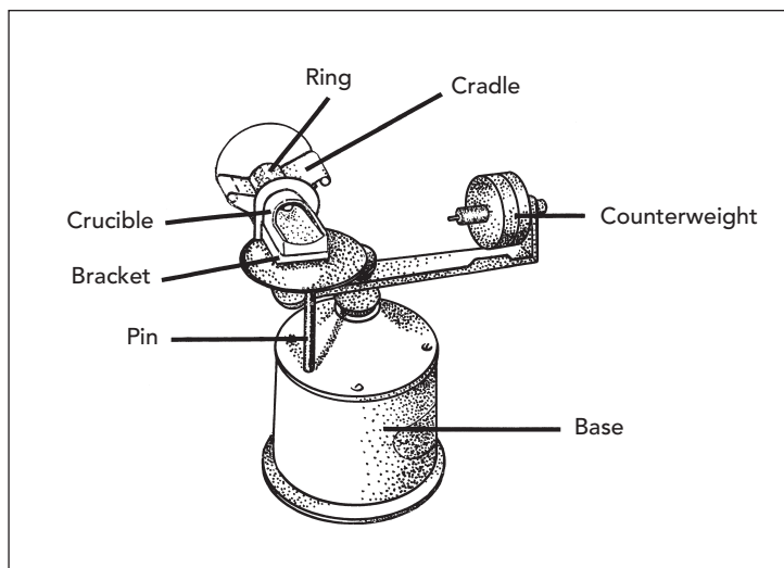
Fig 20-11 Centrifugal casting machine.
