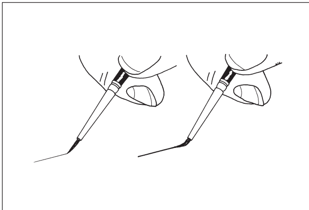
Fig 16-35 The cutting electrode should be used with the same light pressure used to draw a straight line with a brush without bending it ( left ). The pressure exerted on the brush on the right would be excessive.
