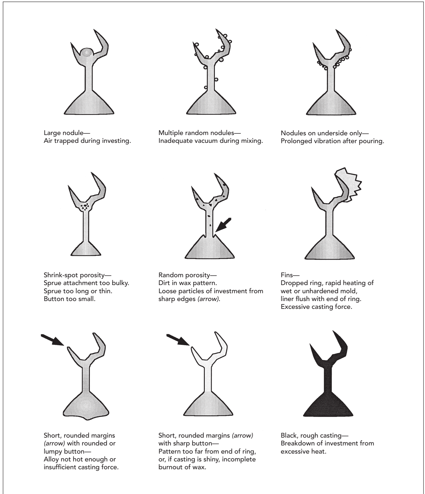
Fig 20-18 Some common casting defects and their causes.
