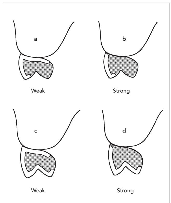
Fig 25-58 (a) A pontic with a short occlusogingival dimension may be too weak with a ceramic ridge contact. (b) It could be strengthened by changing the ridge contact to metal. (c) A pontic may be weakened by covering the occlusal surface with porcelain. (d) The loss of metal bulk can be compensated by using a metal ridge contact.
