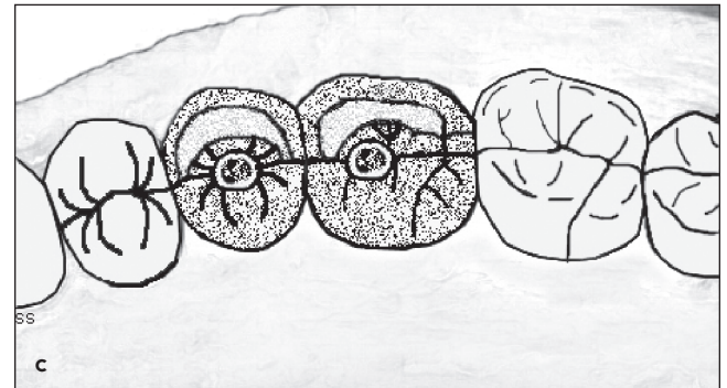
Fig 29-18 (a) Occlusal view of full-contour wax-up showing lingual screw access hole. (b) Buccal view of full-contour wax-up of the implant-retained restoration. (c) Occlusal view of wax pattern with buccal and occlusal buccal cusp reduction. Note that there is no occlusal wax reduction around the abutment screw access holes.
