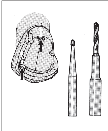
Fig 11-43 Pinholes: no. 1/2 round bur and 0.675-mm twist drill.
