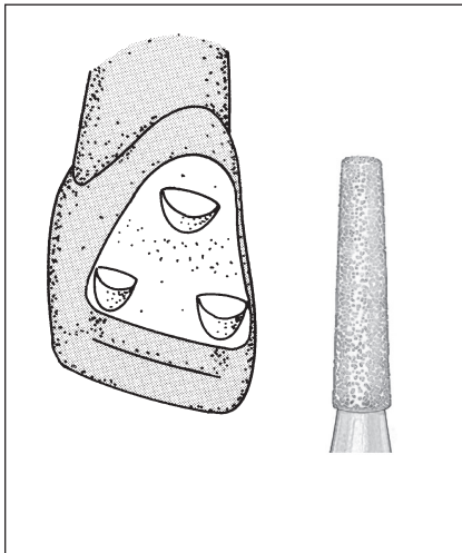
Fig 11-55 Countersinks: flat-end tapered diamond.
