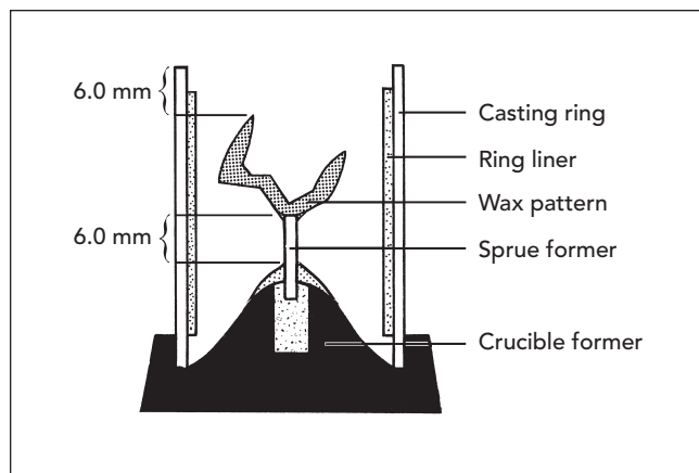
Fig 20-4 Wax pattern ready for investing.
