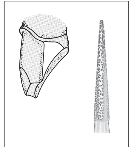
Fig 10-22 Initial proximal reduction: medium-grit long needle diamond.
