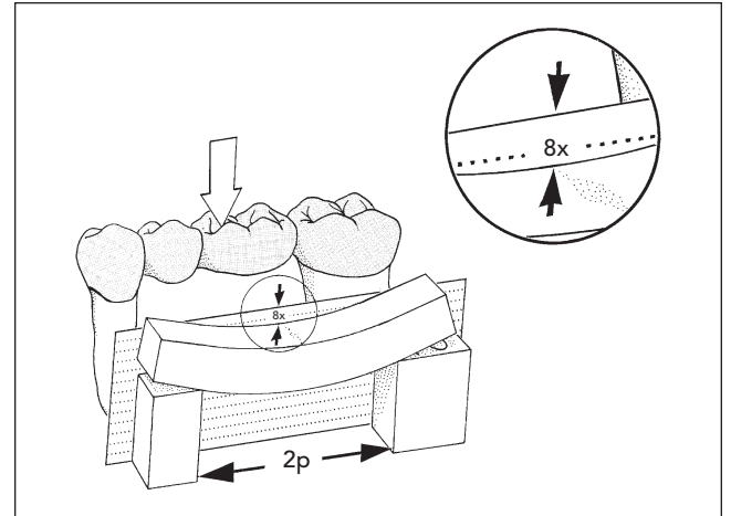
Fig 7-14 The deflection will be eight times as great ( 8x ) if the span length is doubled ( 2p ).
