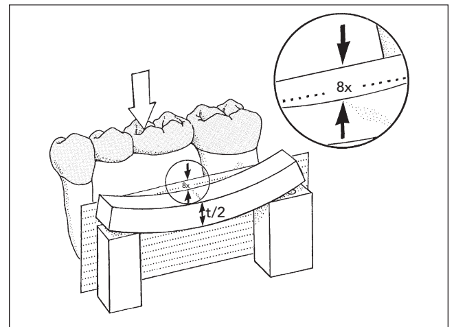
Fig 7-17 There will be eight times as much deflection ( 8x ) if the thickness is decreased by one-half ( t/2 ).
