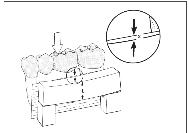
Fig 7-16 There is one unit of deflection ( x ) for a pontic with a given thickness ( t ).
