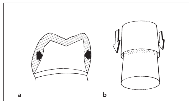
Fig 9-1 An extracoronary restoration (a) uses opposing external surfaces for retention (b).
