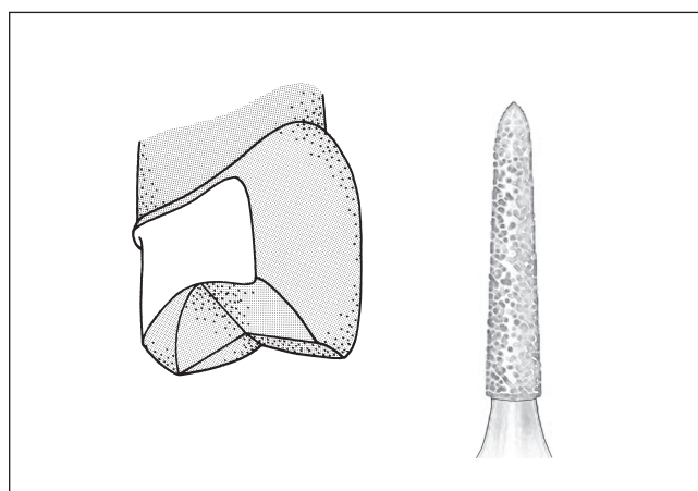
Fig 11-6 Axial finishing: fine-grit tapered torpedo diamond.
