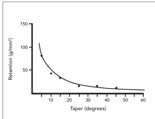
Fig 9-4 As taper increases, retention decreases. (Modified from Jorgensen 4 with permission.)
