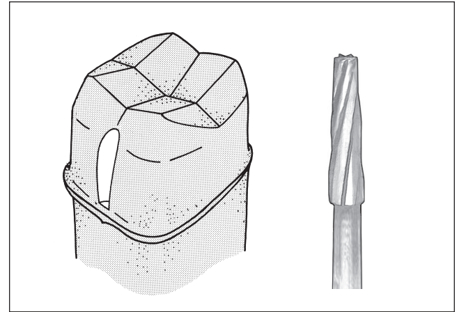
Fig 10-6 Seating groove: no. 171L bur.
