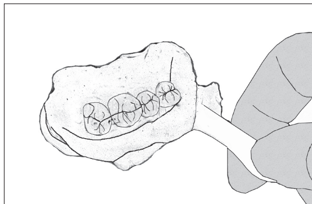
Fig 15-56 Dual-arch impression.
