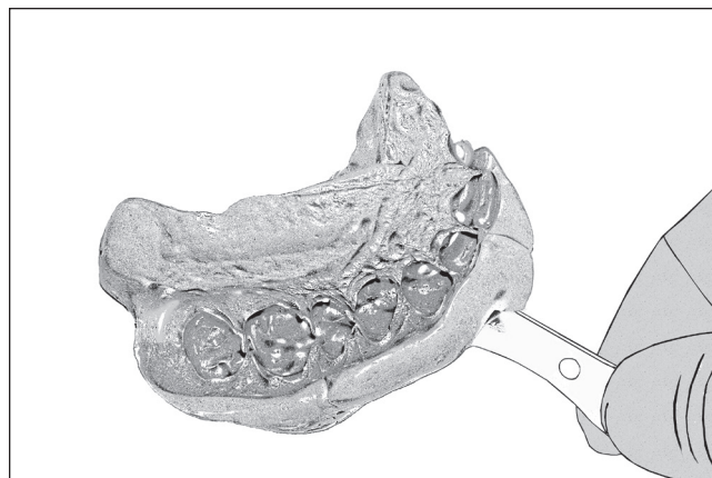
Fig 17-29 Quadrant overimpression.
