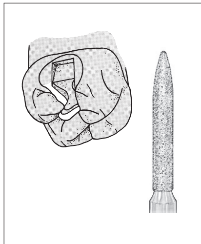
Fig 12-7 Isthmus bevel: fine-grit flame diamond.
