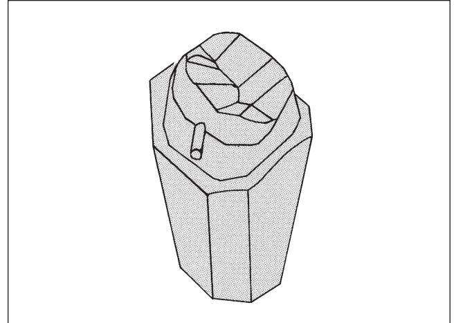
Fig 18-5 A properly trimmed die handle is slightly larger in diameter than the preparation.
