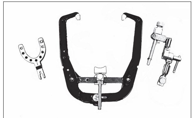
Fig 5-1 The components of a QuickMount facebow are (left to right) a bite fork, the facebow with the nasion relator, and the Quick Lock Toggle assembly.
