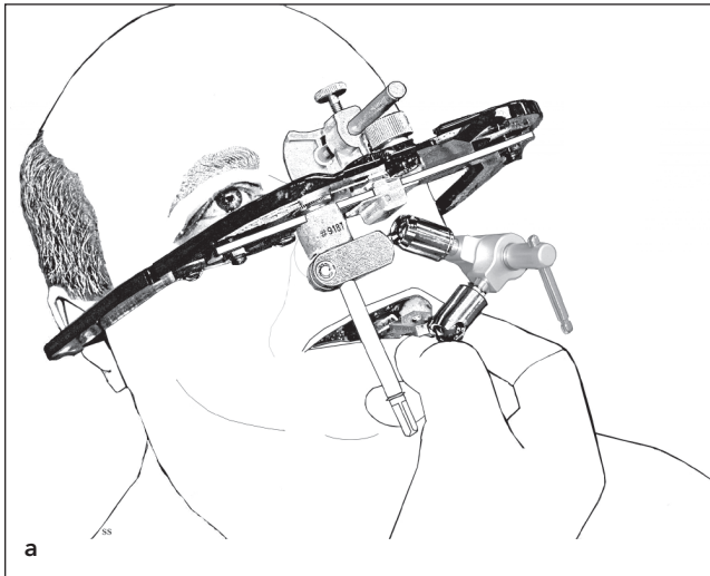
Fig 5-7 The Quick Lock Toggle is slipped into the slot on the bite fork (a), and the thumbscrew is tightened (b).
