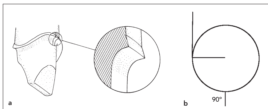
Fig 9-29 Chamfer finish line demonstrated on a full veneer crown preparation.
