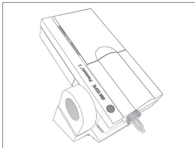
Fig 17-74 Automix machine.
