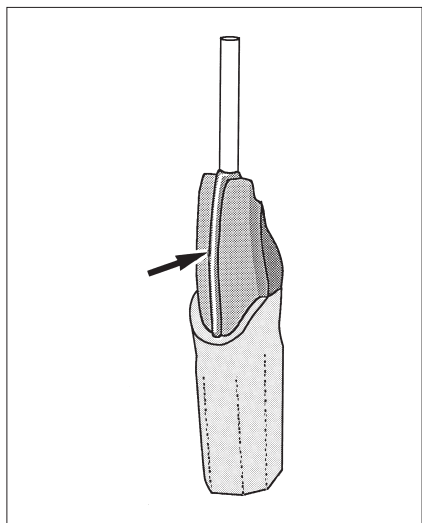
Fig 20-19 Castability of a thin cutback area is improved by the addition of an internal sprue (arrow).
